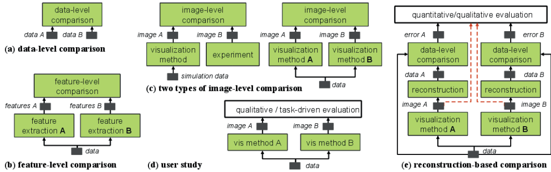
Figure 1: Comparative visualization models based on (a) differences on the data level, (b) differences in extracted features, (c) different visualizations, (d) user studies, and (e) the reconstructability of the underlying data.
