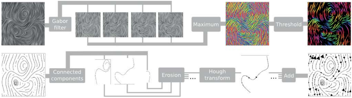
Figure 4: Reconstruction pipelines: (top) The reconstruction of texture-based visualizations uses Gabor filters to quantify local orientations of the texture. (bottom) The reconstruction of line-type structures is based on the Hough transform.
