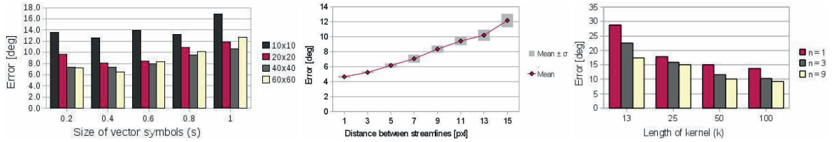
Figure 8: Errors for the three techniques (left to right: vector glyphs, streamlines, and LIC) and different parameter settings.
