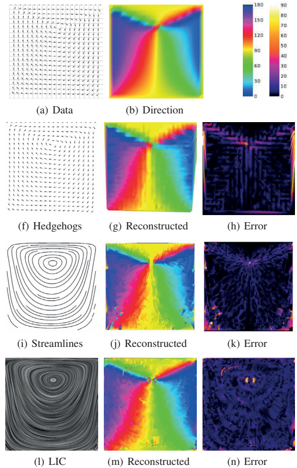
Figure 6: Reconstruction of the cavity dataset: Fig. (a) shows the original grid along with the normalized vector data. A colormap of the direction of the vector field is given in (b). (f,i,l) Three visualization techniques and (g,j,m) the reconstructed directions. (h,k,n) The difference of the directions of the original and the reconstructed field in degrees.
