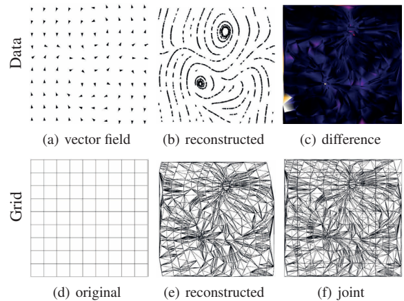
Figure 5: Error computation: To compare the (a) original data and the (b) reconstructed values, a joint version of the two grids (d) and (e) has to be computed. The joint grid (f) comprises all vertices and edges as given in (d) and (e).
