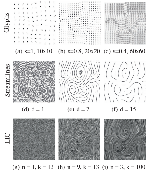
Figure 9: Visualizations with different parameters.
