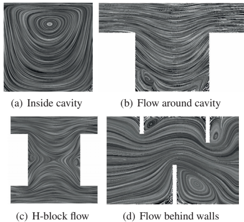
Figure 3: Simulated CFD datasets
