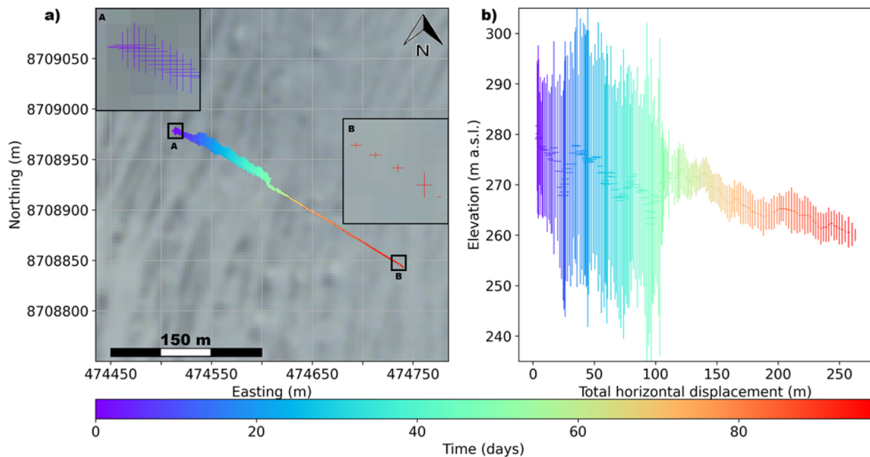
Figure 3. Position of seismic station BH3 on borebreen over time mapped as (a) Easting and northing in UTM coordinates; (b) total horizontal displacement and elevation change. The cross centres mark the mean coordinates values in each 12-hour-long window, the cross's arms' size shows standard deviation (note different XY scales in b), and the colour shows the time elapsed since 10 April 2024. As a background in (a) a satellite photo from 11 September 2023 is used with visible surface crevasses across the flowline. Two insets a and b in (a) show zoomed-in 20 \times 20 m sections of the areas marked with black rectangles.
