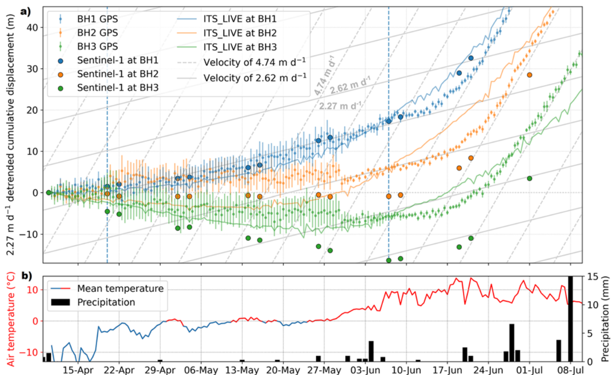
Figure 6. (a) Cumulative displacement detrended by a linear trend of 2.27 \text{ m d}^{-1} , as derived from satellite observations at BH2 (red shading in Figure 4c) (i.e. negative slope informs about sliding slower than 2.27 \text{ m d}^{-1} ). sentinel-1 data are shown as large dots. GPS data are represented by small dots with uncertainty, and ITS_LIVE data are plotted with lines. Blue, orange and green colours indicate BH1, BH2 and BH3 sites, respectively. The opaque grid of solid and dashed grey lines indicate displacements corresponding to sliding velocities of 2.62 and 4.74 \text{ m d}^{-1} , respectively. The 4.74 \text{ m d}^{-1} velocity was interpreted as best fit to BH2 data after speed-up (blue shading in Figure 4c), while the 2.62 \text{ m d}^{-1} velocity was fitted to BH1 GPS data prior to speed-up in the interval marked by vertical blue dashed lines. (b) Temperature at Borebreen (blue–red line) and precipitation at Longyearbyen (black bars). The temperature was measured by each BH1–BH3 station and averaged. It may be affected by direct sunlight.
