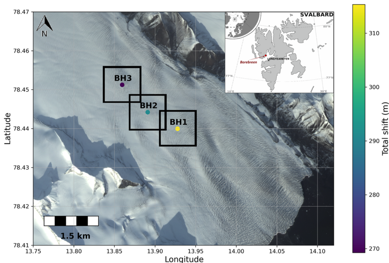
Figure 1. Orthophoto map of the borebreen study area. The dots indicate the positions of seismic stations. The colour of the dots represents the total displacement in the horizontal direction measured by the internal GPS over the time of deployment. The black rectangles mark the area contributing to the Sentinel-1 velocity time series. The baseline is a Planet Labs SkySat photo from 11 September 2023. The inset map in the top right corner presents the location of Svalbard and the location of Borebreen in Svalbard (red dot).
