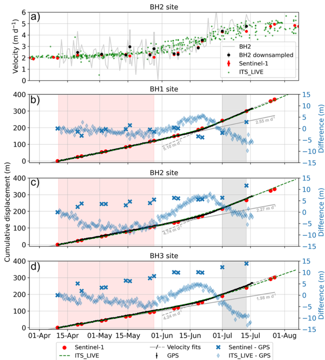
Figure 4. Comparison of satellite and seismic station internal GPS time series. (a) Direct velocity comparison at BH2 area: red dots represent sentinel-1 data, black dots represent downsampled GPS data, the grey curve represents daily averaged BH2 GPS data, and green dots represent ITS_LIVE data; (b–d) cumulative displacements along the flowline at the sites BH1, BH2, and BH3, respectively: red dots represent sentinel-1 data, black dots show GPS data in 12 hour averaged windows with uncertainty, and green dashed line represents ITS_LIVE data. Grey solid and dashed lines represent displacements from sliding velocities indicated at respective panels, that were fitted to satellite data (red shading) and GPS data (grey shading), respectively. The difference between sentinel- and GPS-derived displacement is shown with blue crosses and between ITS_LIVE and GPS with blue diamonds (right-hand side axis).
