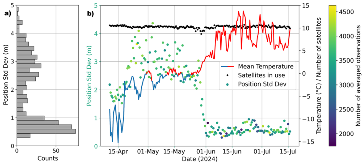
Figure 5. Seismic station GPS horizontal positioning precision along the flowline. (a) Histogram of the qc-ed standard deviation values in each 12 hour window for all three stations; (b) The qc-ed standard deviation over time marked with coloured scatter points. The colour of each point corresponds to the number of samples used during the averaging. The daily temperature at Borebreen measured by each BH1–BH3 station and averaged is marked by blue–red line. It may be affected by direct sunlight. Additionally, the average number of satellites used for position determination in each 12 hour window is plotted with black dots.
