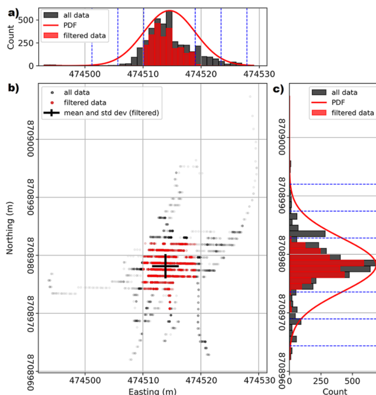
Figure 2. Distribution of Northing and Easting (UTM) coordinates in the first 12-hour-long analysis interval at the BH3 (top) site. (b) A scatter plot showing all (black dots) and filtered data (red dots) with a black error bar representing the mean and standard deviation recalculated for the filtered (red) dataset. Data points are plotted with 90% transparency; (a) and (c) Northing and Easting coordinates, respectively, distributions presented as histograms with grey bars for all the data and red bars for filtered data. The red curve represents the probability density function (PDF) inferred for all the data (scale is not presented) and dashed blue lines represent the limits of inferred pdf's one, two, and three sigma intervals of the whole dataset.
