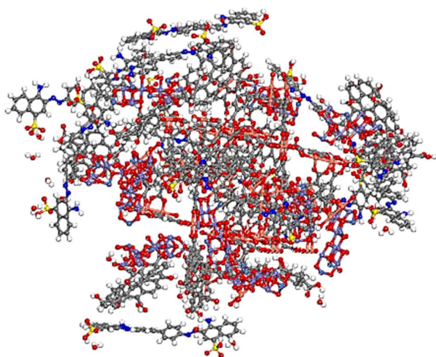
Fig. 20 The lowest adsorption configuration of adsorption of CR molecules on \text{NiFe}_2\text{O}_4(311)@HKUST-1/\text{GO} by Monte Carlo simulation.
