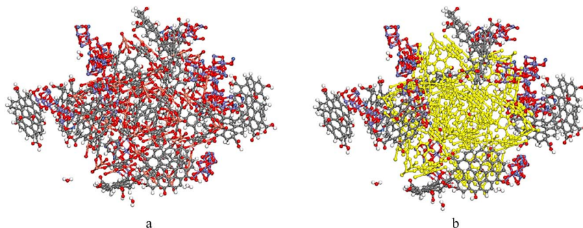
Fig. 19 (a and b) The adsorption of GO on \text{NiFe}_2\text{O}_4(311)@HKUST-1 surface to form \text{NiFe}_2\text{O}_4(311)@HKUST-1/\text{GO} by Monte Carlo simulation.
