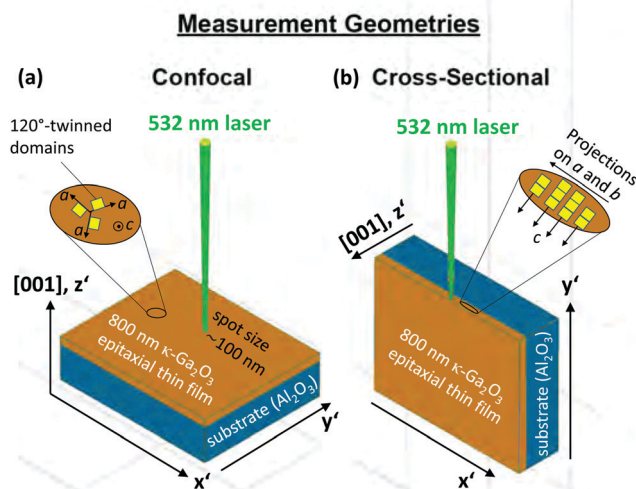
Fig. 3 Schematic illustration of sample setup, plane orientation, and measurement geometry. The (001) plane was accessible in (a) confocal micro-Raman scattering. The z' and x', y' directions of a Cartesian coordinate system are oriented perpendicular to the (001) plane and parallel to the edges. Spectra recorded in a (b) cross-sectional set-up are acquired by focusing the laser onto the edge (right). The insets indicate (a) the 120° rotation of orthorhombic domains around the c -axis or (b) the columnar c -oriented structure perpendicular to the (001) plane.
