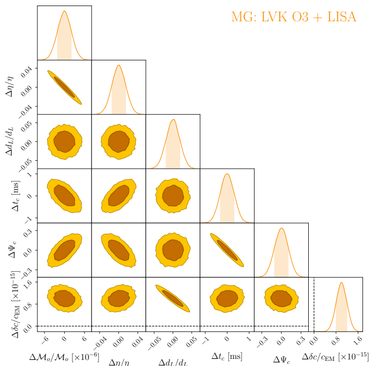
Figure 4. Joint LVK O3 + LISA constrains for an event with m_1 = 36M_\odot , m_2 = 29M_\odot , z = 0.09 , t_c = 0 , \Psi_c = 0 and \delta c/c_{EM} = 10^{-15} .
