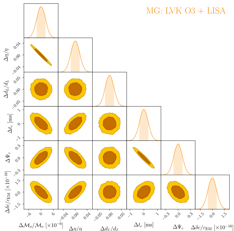
Figure 3. LVK O3 + LISA constrains for an event with m_1 = 36M_\odot , m_2 = 29M_\odot , z = 0.09 , t_c = 0 , \Psi_c = 0 and \delta c/c_{\text{EM}} = 0 .
