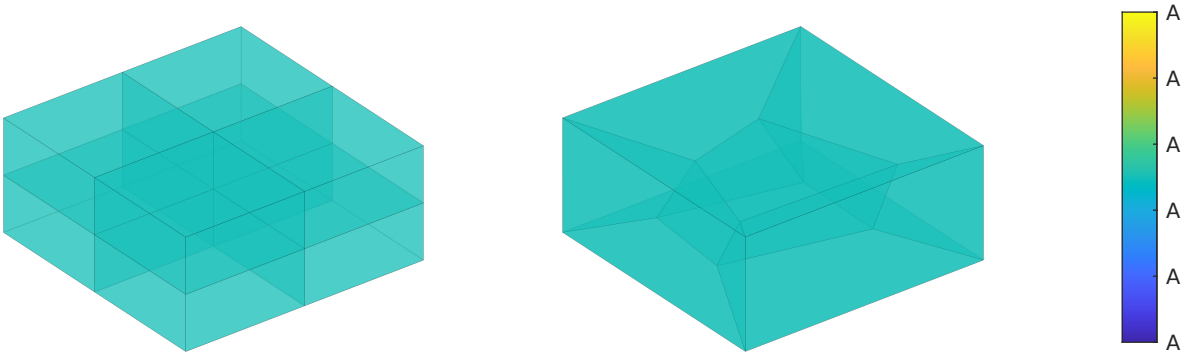
Figure 4: Temperature distribution \theta [K] resulting from the patch test for the regular and the distorted mesh.
