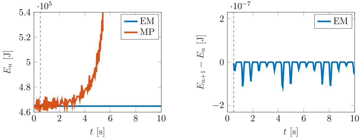
Figure 11: Left: Evolution of the total energy resulting from the rotating cross-shaped body example over the course of the simulation computed using both the energy-momentum scheme (EM) and the midpoint rule (MP). Right: Incremental differences of the total energy from one time step to the next.
