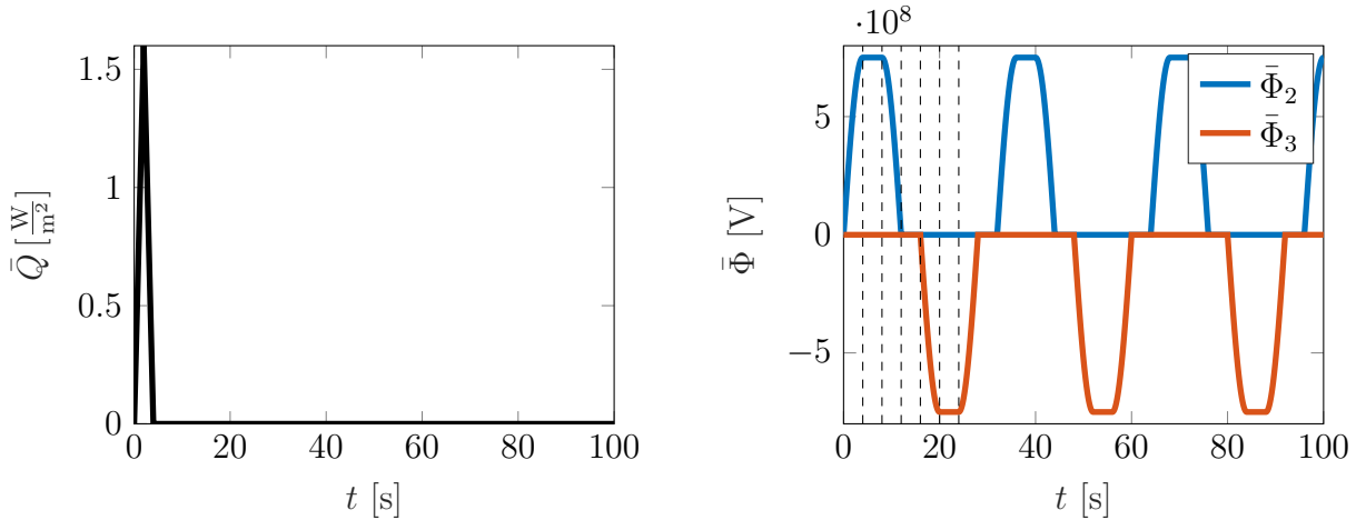
Figure 15: Heating of the pump with \bar{Q} (left) and electric potential fields \bar{\Phi}_2 and \bar{\Phi}_3 for the pumping process (right) employed for microfluidic pumping device example.
