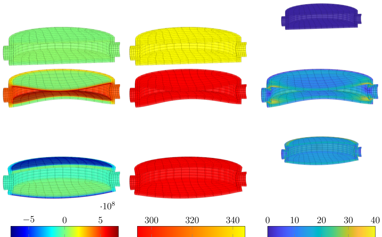
Figure 17: Snapshots of the microfluidic pumping device with electric potential field \Phi [V] (left), the absolute temperature field \theta [K] (mid), and von Mises stress \sigma_{vM} [Pa] (right) at t = 0 s (top), t = 6 s (mid), and t = 22 s (bottom).
