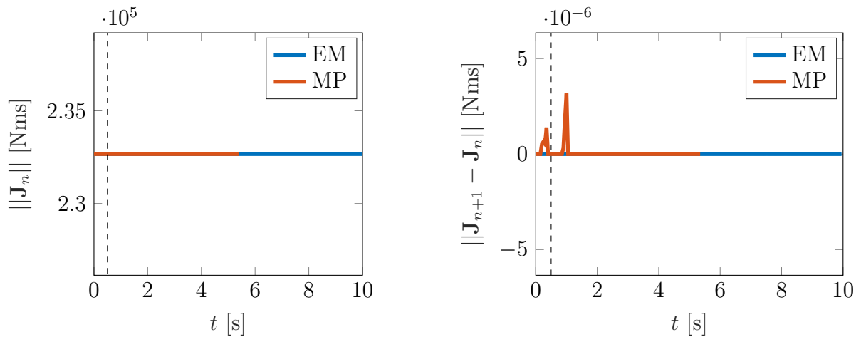
Figure 10: Left: Evolution of the total angular momentum resulting from the rotating cross-shaped body example over the course of the simulation computed using both the energy-momentum scheme (EM) and the midpoint rule (MP). Right: Incremental differences of the total angular momentum from one time step to the next.
