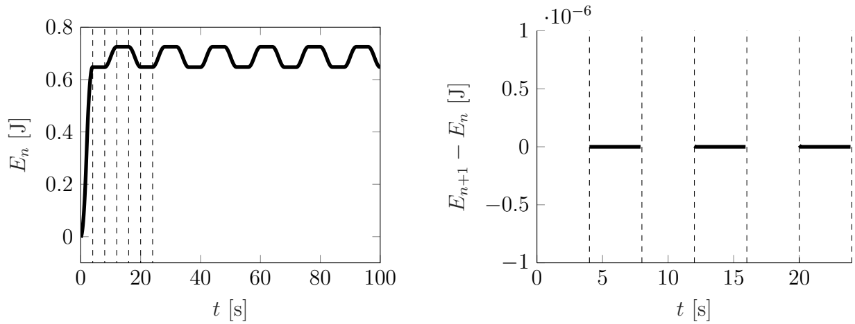
Figure 16: Total energy of the microfluidic pumping device (left) and energy difference (right) for the first pumping cycle, see also Fig. 15 (right).
