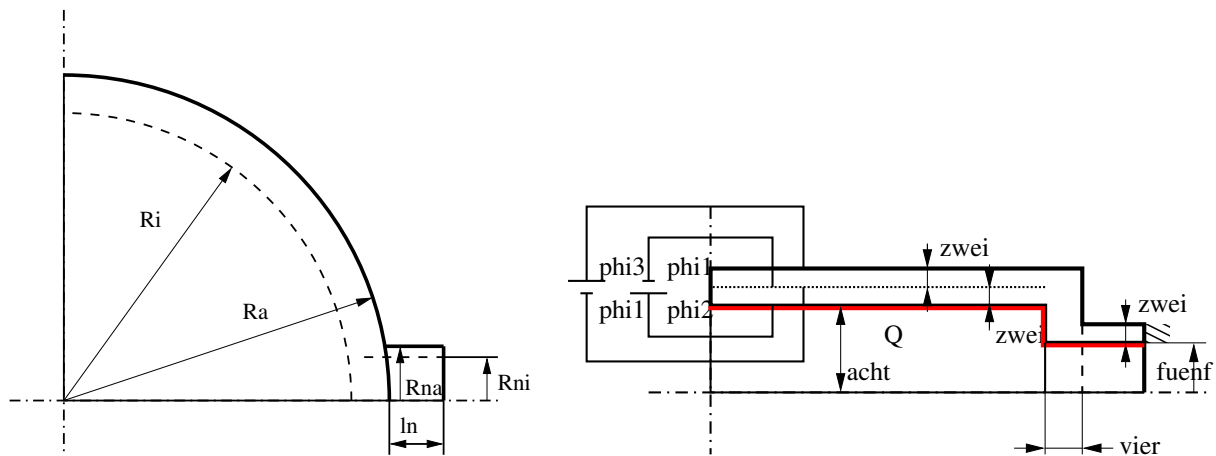
Figure 14: Top view (left) and side view (right) including mechanical (symmetry lines and hatching), electrical ( \Phi_{1-4} ), and thermal ( Q ) boundary conditions employed for microfluidic pumping device example.
