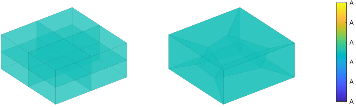
Figure 5: Electric potential distribution \Phi [V] resulting from the patch test for the regular and the distorted mesh.
