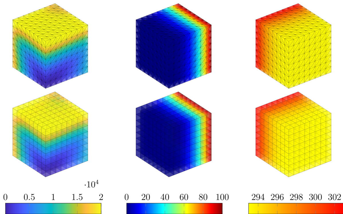
Figure 7: Von Mises stress \sigma_{vM} [Pa] (left), electric potential \Phi [V] (mid), and absolute temperature \theta [K] (right) for P2P1^d (top), and H2^cH1^d (bottom) meshes, respectively.
