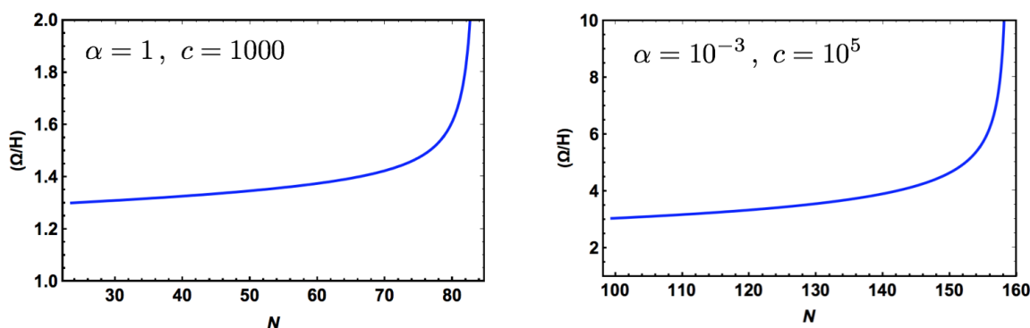
Figure 6. Turning rate in the original EGNO model for two sets of parameters. On the left, we use the parameters and initial conditions given in figure 3 and find \omega(N_{\text{end}}) \simeq 3 , where N_{\text{end}} is the end of inflation, i.e. \epsilon = 1 . On the right, we use \alpha = 10^{-3} , c = 10^5 to increase the turn rate up to \omega(N_{\text{end}}) \simeq 42 .
