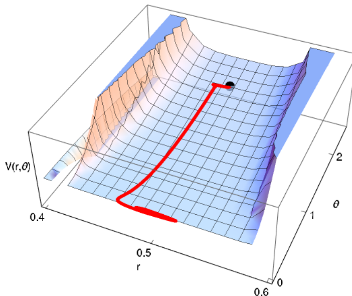
Figure 3. EGNO potential and inflationary trajectory for the parameters \alpha = 1 , a = 1/2 , M = 10^{-3} , c = 1000 , and p = 0 as in the original model [44]. The initial conditions are r_{\text{ini}} = a , \theta_{\text{ini}} = 5a\sqrt{2/3} , yielding N_{\text{tot}} = 87 .
