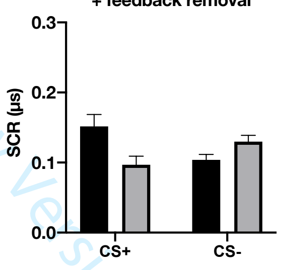
d Extinction + feedback removal
