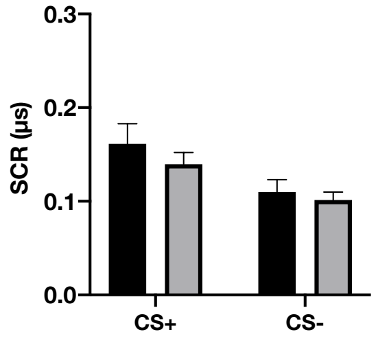
d Extinction + feedback removal
