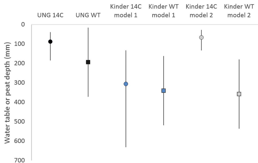
Figure 10. Comparison of modeled water table (squares) and depth of peat (circles) associated with the mean modeled 14 C age of dissolved organic carbon for each catchment, including both model versions for Kinder River. Error bars are 2 × RMSE of the water table model tested against the intact data set (Figure 7) (WT) and the interquartile range of the source depth distribution from the 14 C model.
