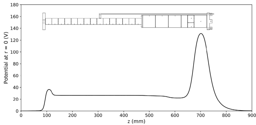
Fig. 6. Schematic illustration of the first two stages of the BGT, together with the calculated axial trapping potential on the z-axis, in the centre of the electrodes. The last but one electrode, going from left to right, is segmented in four parts and this is where the four RW voltages are applied. Nitrogen gas is injected into the middle of the first stage using the delivery pipe shown, whilst carbon dioxide is inserted into the second vacuum cross (see Fig. 2) and subsequently diffuses into the second and third stages.
