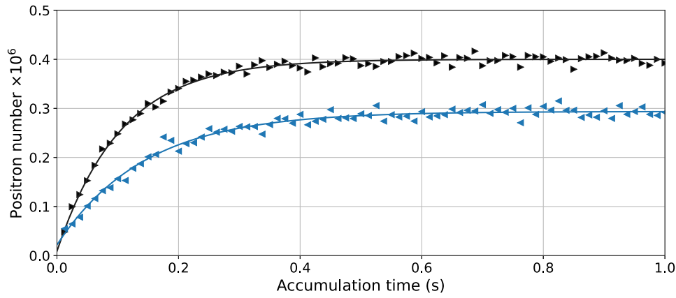
Fig. 8. Accumulation in the second stage without using the RW. The blue points ( \blacktriangleleft ) are measurements taken while there was only nitrogen gas inserted into the system. The fitted line gives \tau = 0.144(6) s and R = 1.9(1) \times 10^6 e ^+ s ^{-1} . The black points ( \blacktriangleright ) were taken with both nitrogen and carbon dioxide present and with fitted values of \tau = 0.105(3) s and R = 3.7(2) \times 10^6 e ^+ s ^{-1} .
