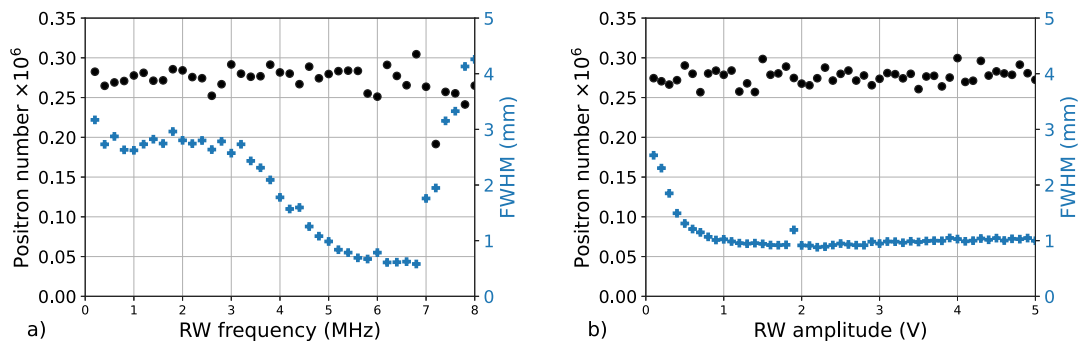
Fig. 11. (a) Positron number ejected from the BGT's third stage (•) and FWHM of the positron cloud imaged on the MCP (✚) (a) as a function of the RW frequency, with a RW amplitude of 1 V; (b) as function of the RW amplitude, with a RW frequency of 5 MHz.
