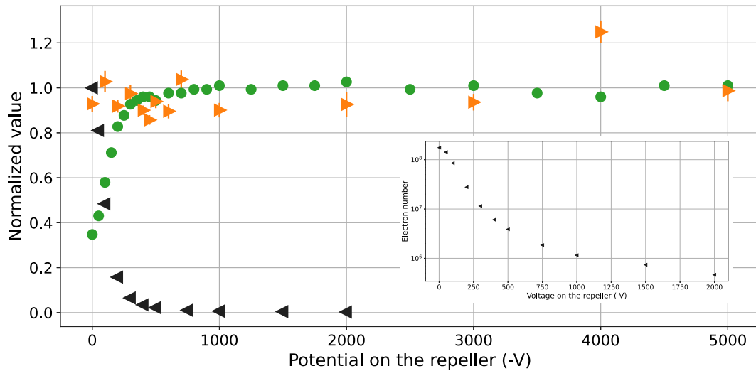
Fig. 5. Normalised values for the number of electrons ( \blacktriangleleft ), positron trapping rate ( \bullet ) in the second stage of the BGT and the parallel energy width of the positrons ( \blacktriangleright ). The RW was on during the accumulation using a frequency of 2.4 MHz and a voltage on the electrodes of 1 V. Inset: number of electrons on a log-lin scale. The linac frequency was 200 Hz.
