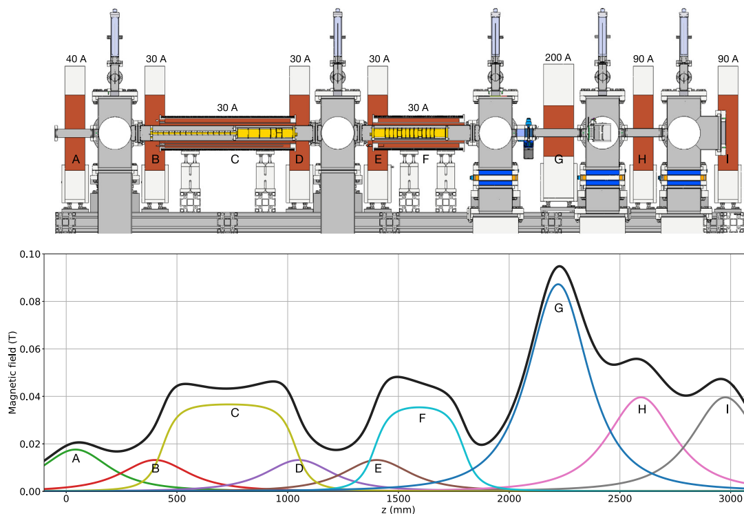
Fig. 2. Cross section of the three stage buffer gas trap (top) where the upstream side is on the left. There are two trapping areas, the first two stages (yellow, left) of the trap are inserted in a vacuum tube which is inside a solenoid between the first and second pumping stages, and similarly the third stage (yellow, right) is positioned between the second and third pumping stations. There are seven coils providing the magnetic field between the trap areas to guide the positrons. The numbers above the coils and the solenoids are the currents used to power the magnet. The calculated magnetic field along the axis of the system is shown in the bottom figure. The black line is the total field while the other coloured lines are the fields originating from the individual coils and solenoids (labelled A to I).
