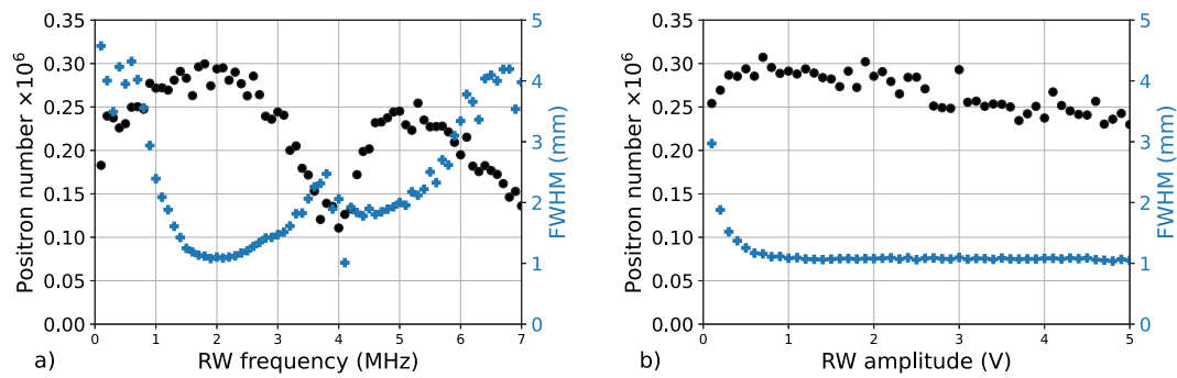
Fig. 9. Positron number ejected from the BGT's second stage ( \bullet ) and FWHM of the positron cloud imaged on the MCP ( \blackstar ) after 100 ms accumulation. (a) as a function of the RW frequency, with a RW amplitude of 1 V; (b) as a function of the RW amplitude, with a RW frequency of 2 MHz.
