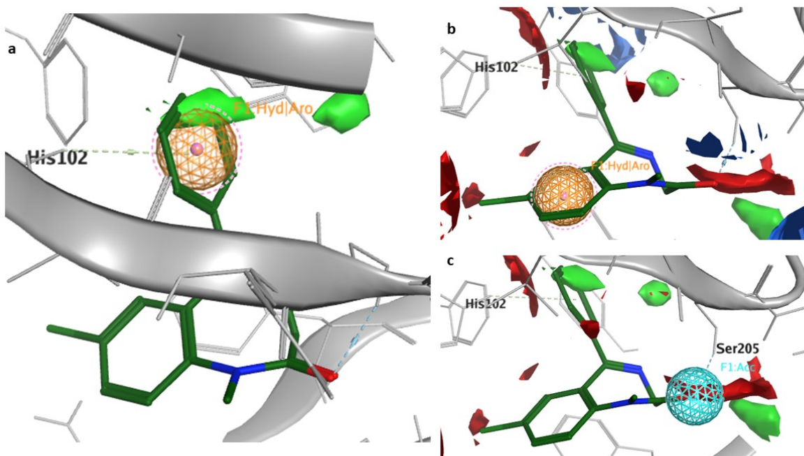
Figure 1 Ligand pharmacophore features taken into consideration for the scaffold hopping exercise
