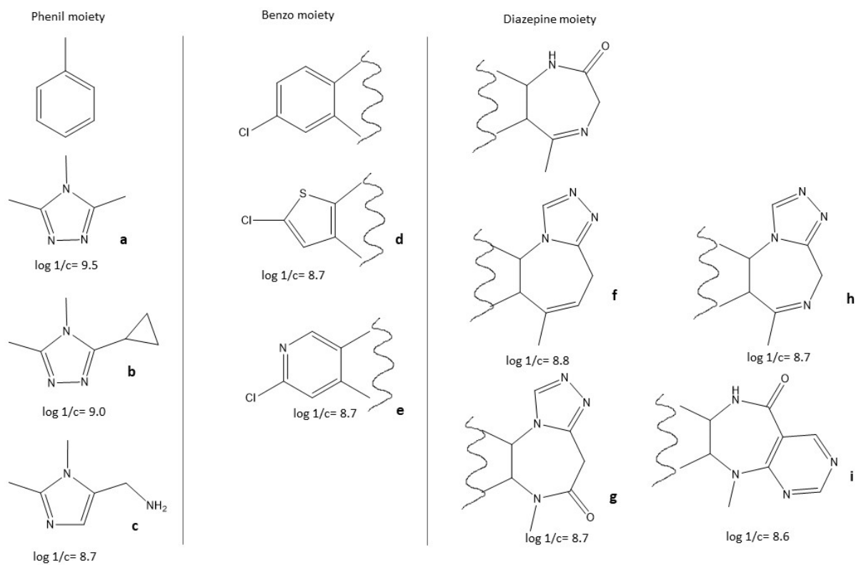
Figure 1 MedChem and Scaffold Replacement top scoring moieties
