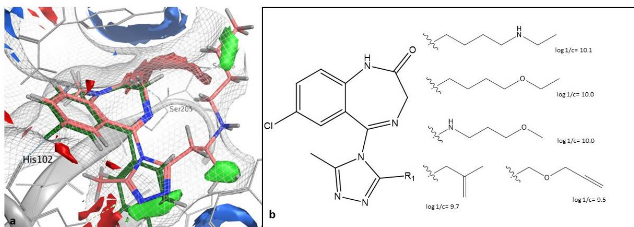
Figure 1 (a) 3D representation of the new scaffold created and its adopted conformation inside the binding pockets. b) the predicted activities retrieved from “Add Group to Ligand” exercise on the C2 of the triazole pendant ring
