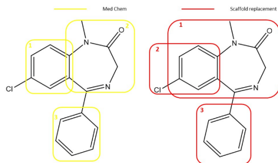
Figure 1 Three major moieties (1,2,and 3) for the MedChem (yellow) and Scaffold Replacement (red) studies
