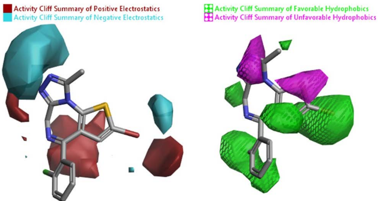
Figure 1 Visual representation of the generated 3D Field QSAR model
