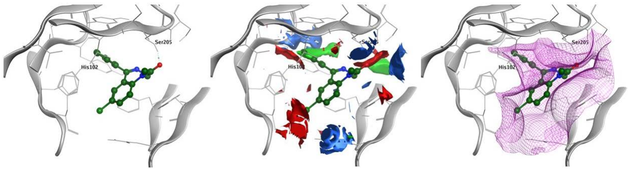
Figure 1 Diazepam bound in its active conformation in the GABA-AR (6HUP 35 ).
