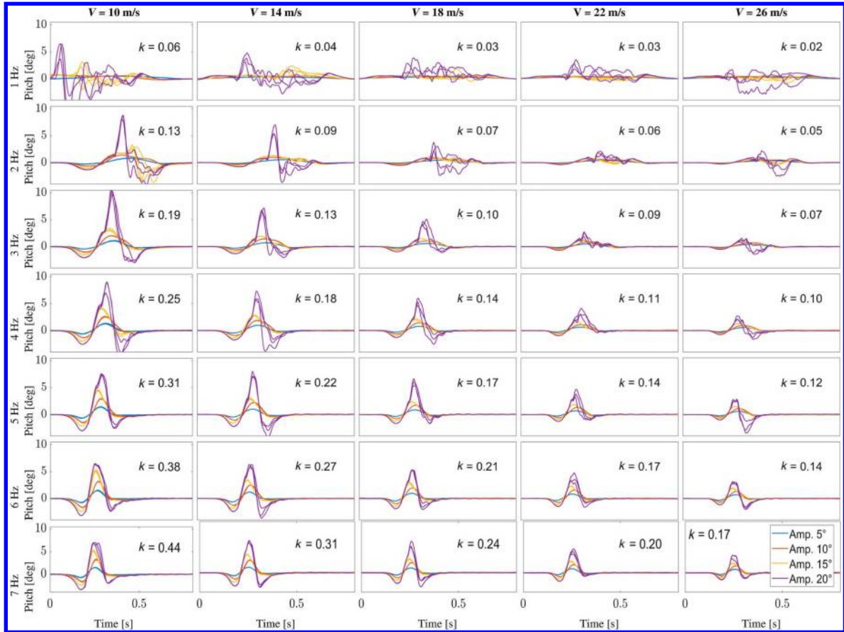
Fig. 7 Discrete gust vane rotations amplitude of 5, 10, 15, and 20°, 1–7 Hz rotation frequency. Each case was repeated three times, and all data are plotted.
