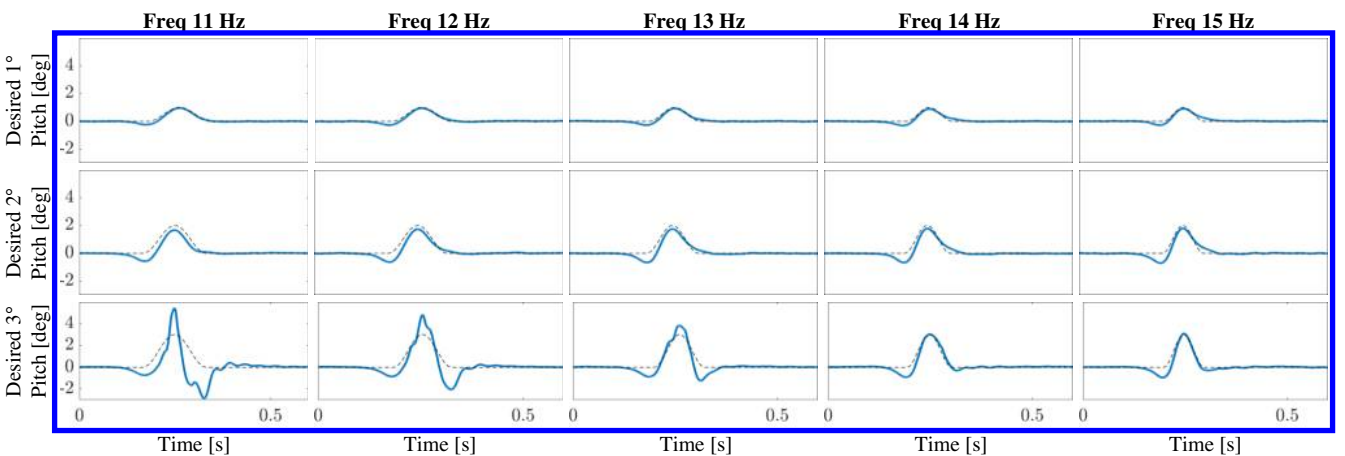
Fig. 20 Discrete gust vane rotations with desired angle of attack 1, 2, and 3°, and frequency 11–15 Hz and ideal “1-cos” gust at 18 m/s (black dashed line).
