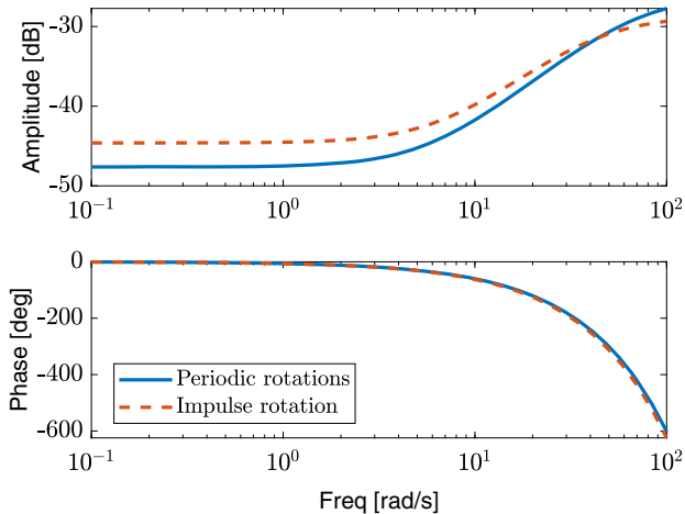
Fig. 18 Comparison of identified transfer functions at 18 m/s.
