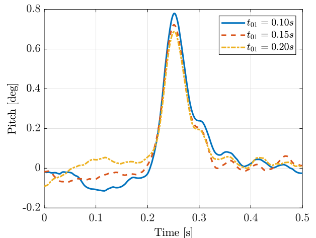
Fig. 24 Proposed method, effect of t_{01} on the gust produced.
