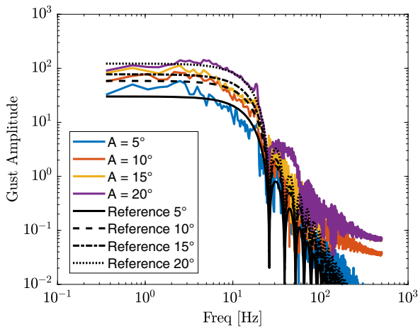
Fig. 29 Frequency content of discrete gusts obtained at 18 m/s, frequency of 13 Hz, by the proposed method for amplitude of 5, 10, 15, and 20° (color lines) and frequency content of the equivalent exact discrete gusts with the same gust wavelength and maximum amplitude (black lines).
