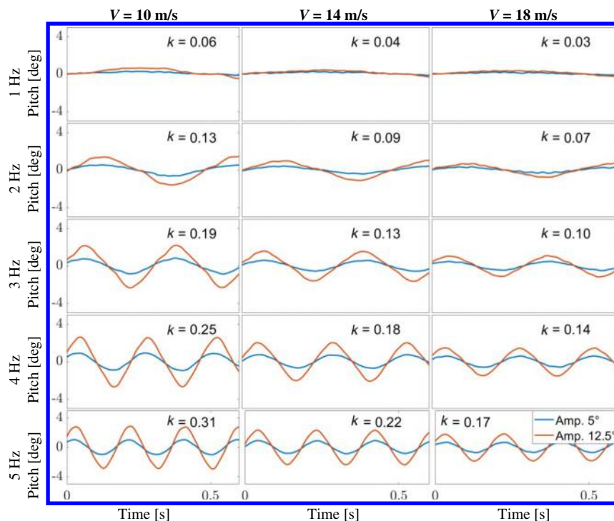
Fig. 10 Continuous gust for vane rotations amplitude of 5 and 12.5^\circ , at 1–5 Hz.
