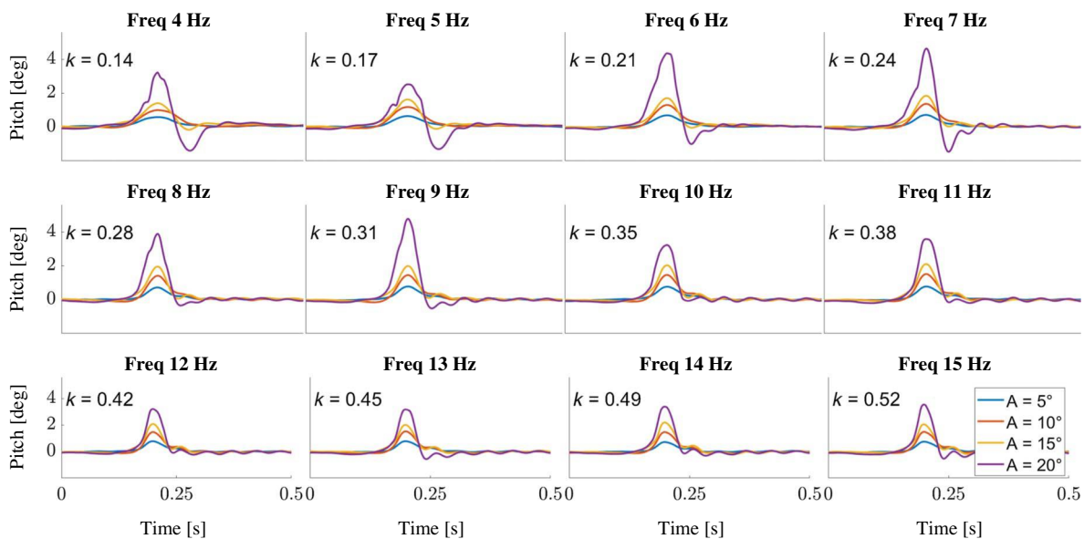
Fig. 27 Proposed method to parameterize the discrete gust vane rotation for amplitude of 5, 10, 15, and 20°, and frequencies of 4–15 Hz.
