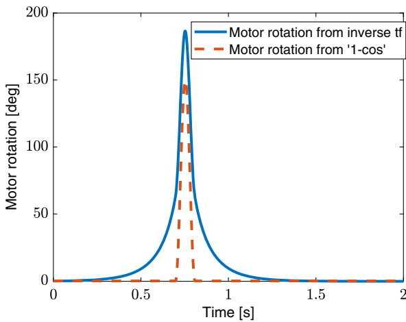
Fig. 21 Comparison motor rotation found from inverse transfer function and “1-cos”.
