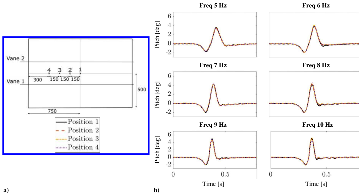
Fig. 12 Gust uniformity at different horizontal locations (a) and discrete gusts at each location (b).
