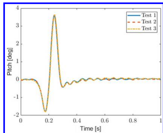
Fig. 6 Discrete gust, evaluation repeatability.
