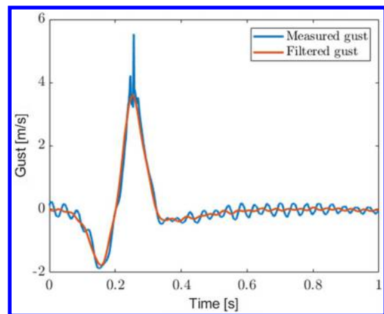
Fig. 5 Measured gust and filtered gust.
