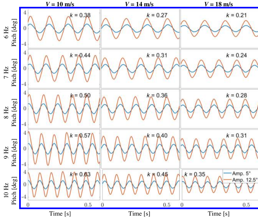
Fig. 11 Continuous gust for vane rotations amplitude of 5 and 12.5°, at 6–10 Hz.
