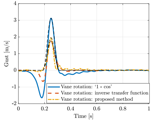
Fig. 30 Discrete gust at 8 Hz from “1-cos” vane rotation and vane amplitude 10°, from the vane rotation calculated from the inverse of the transfer function with a desired gust of 2°, and from the proposed method with A = 15^\circ and corresponding ideal “1-cos” gusts (black dashed lines).
