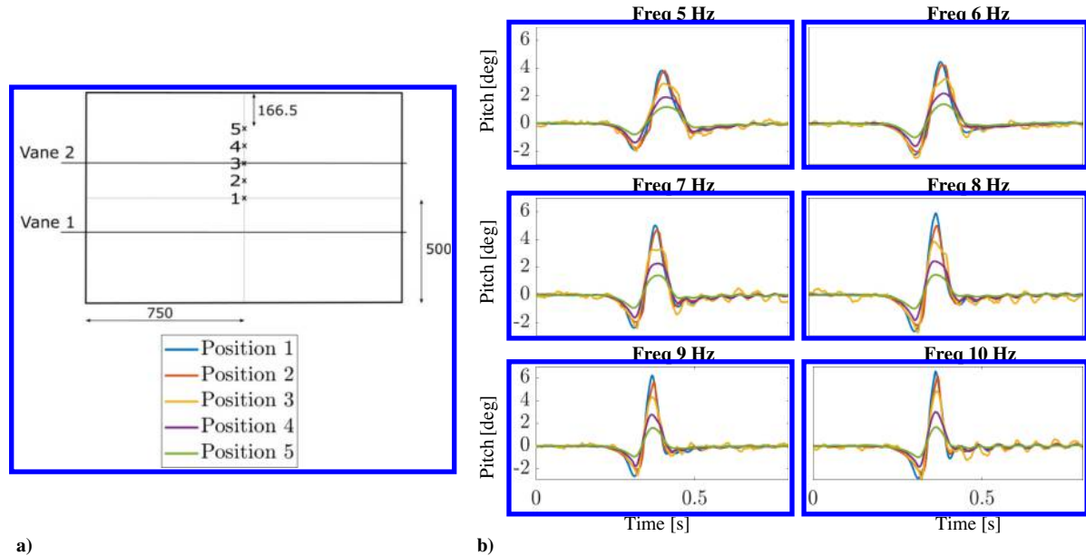
Fig. 13 Gust uniformity at different vertical locations (a) and discrete gusts at each location (b).
