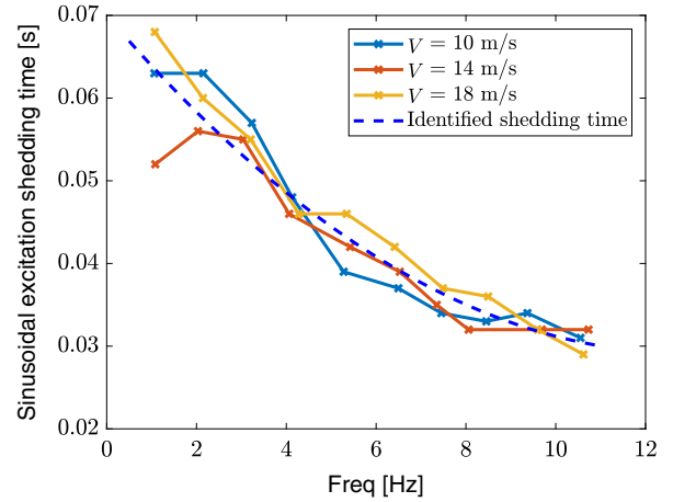
Fig. 16 Experimental and identified shedding times from continuous sinusoidal vane rotation.
