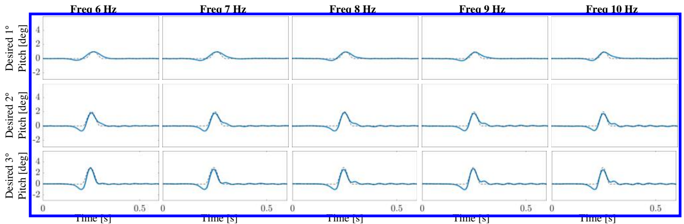
Fig. 19 Discrete gust vane rotations with desired angle of attack 1, 2, and 3°, and frequency 6–10 Hz and ideal “1-cos” gust at 18 m/s (black dashed line).
