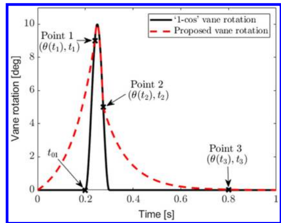
Fig. 23 Proposed method to parameterize the vane rotation.
