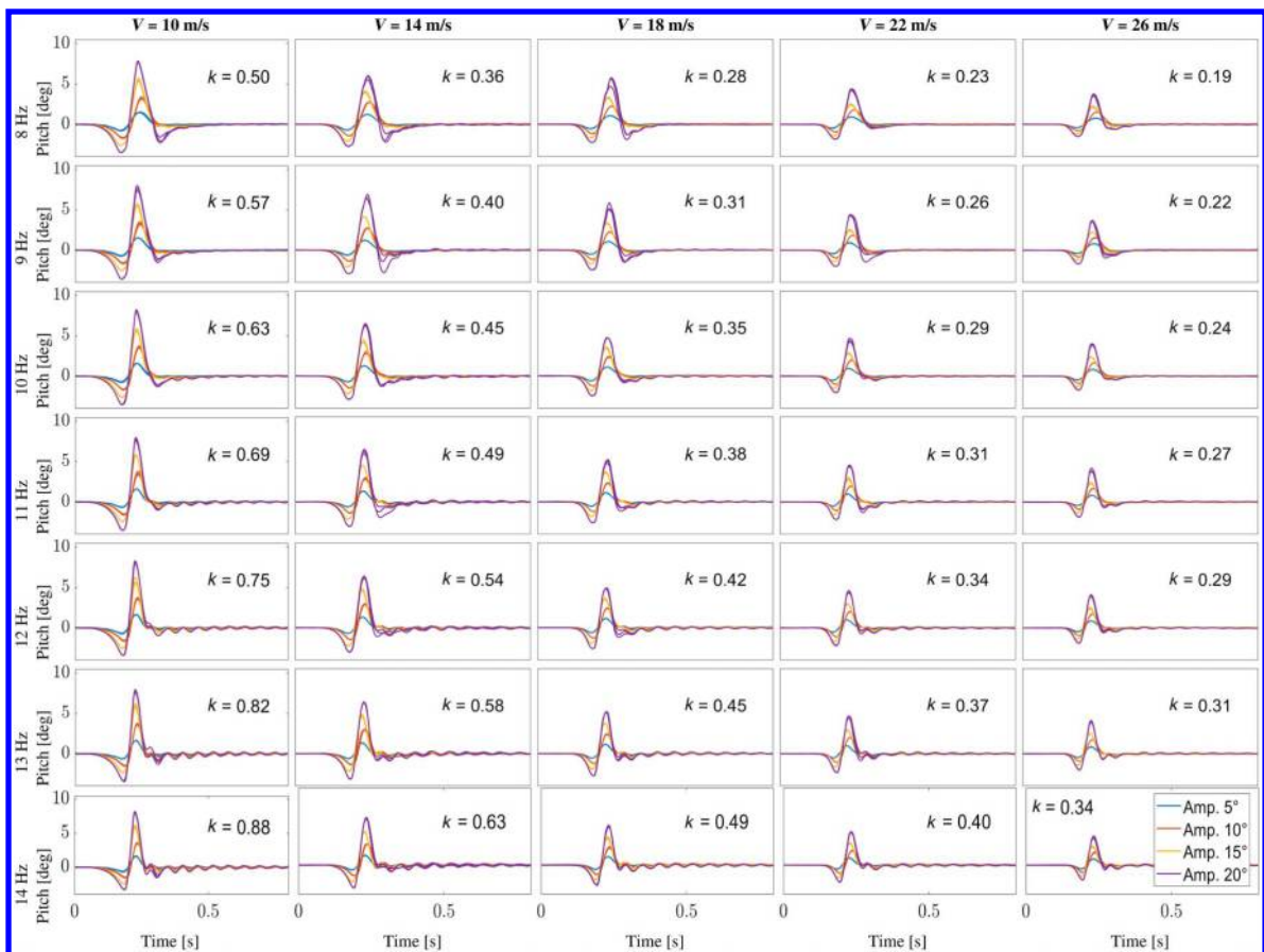
Fig. 8 Discrete gust vane rotations amplitude of 5, 10, 15, and 20°, 8–14 Hz rotation frequency. Each case was repeated three times, and all data are plotted.
