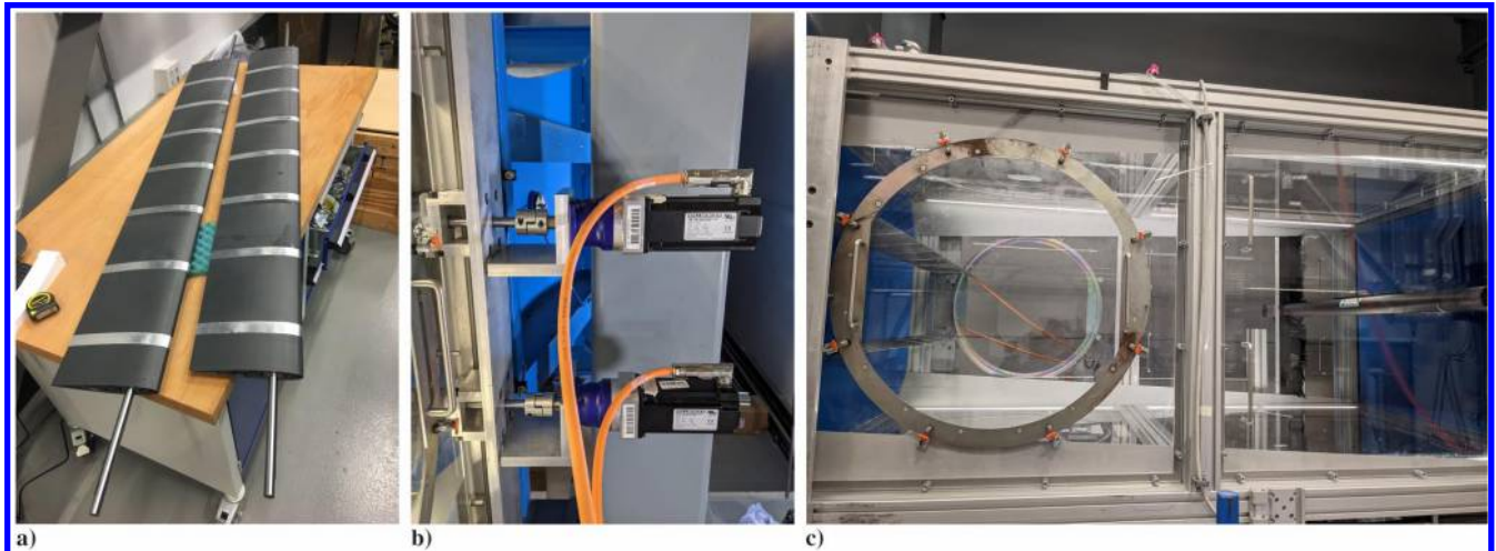
Fig. 4 Vanes (a), motors and gearboxes (b), and vanes in the wind tunnel (c).
