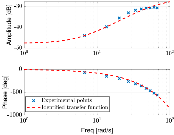
Fig. 15 Identified transfer function from sinusoidal test at 18 m/s.
