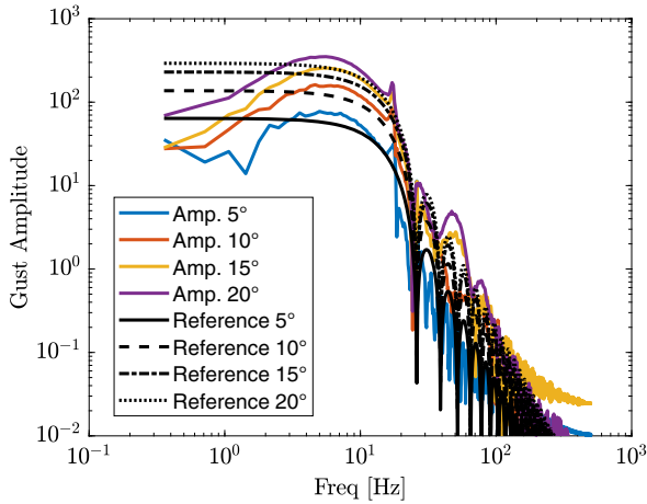
Fig. 28 Frequency content of discrete gusts obtained at 18 m/s, frequency of 13 Hz, by “1-cos” vane rotation for amplitude of 5, 10, 15, and 20° (color lines) and frequency content of the equivalent exact discrete gusts with the same gust wavelength and maximum amplitude (black lines).
