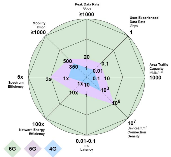
FIGURE 9. 6G Requirements [28], [76], [191].
