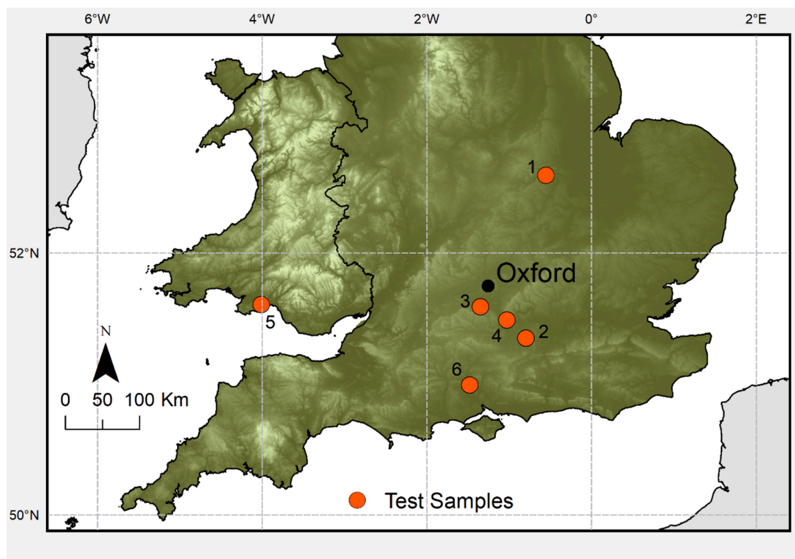
Fig. 1. The location of the samples analysed in this study (red circles). 1. Fineshades (ash); 2. Crowthorne (chestnut); 3. West Hendred (elm); 4. Mapledurham (beech); 5. Clyne (alder); 6. Cuppernham (black poplar). The south central England isotope chronology used as a reference chronology in this study contains samples sourced from across a c. 33 600-km 2 area roughly centred on Oxfordshire.
