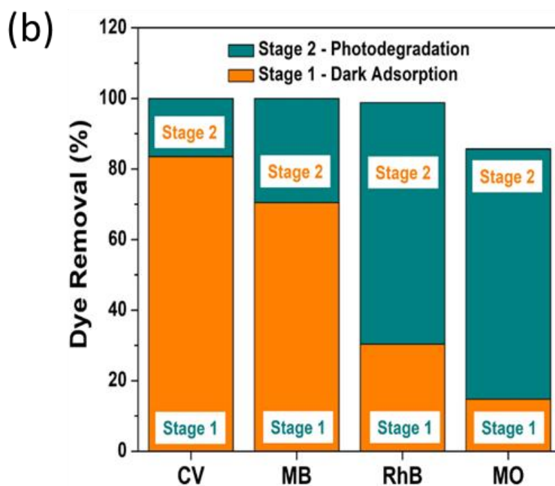
Figure 7. (a) Dark adsorption (stage 1) at TM50%, and photocatalytic degradation (stage 2) at TM2.5% samples. (b) Dye removal efficiency of MB, MO, RhB and CV dyes estimated from Figure 7 (a).
