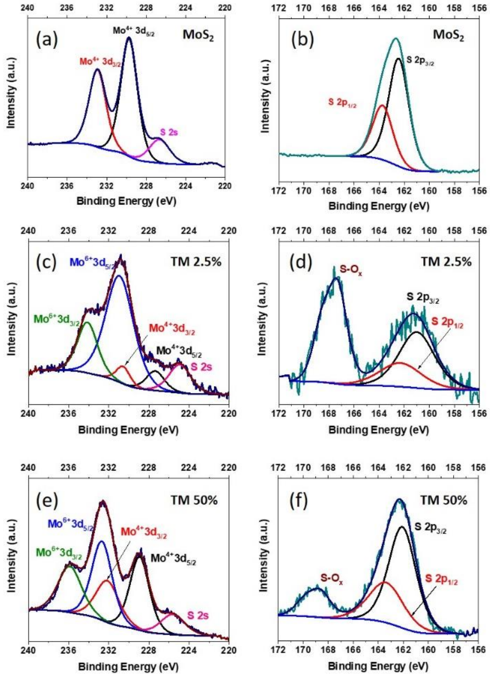
Figure 4. XPS core level spectra of Mo3d and S2p measured at (a) and (b) MoS 2 ; (c) and (d) TM 2.5% (TiO 2 /MoS 2 composite) and; (e) and (f) TM 50% (TiO 2 /MoS 2 composite).
