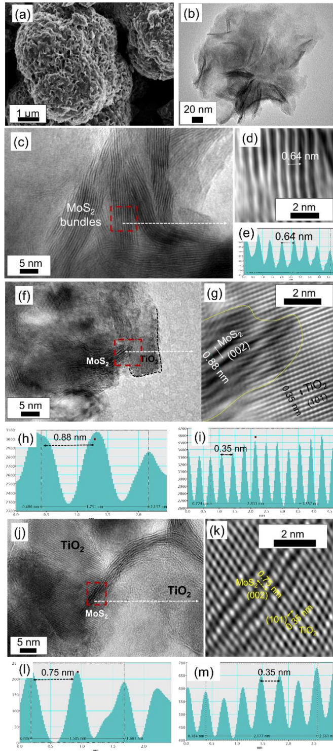
Figure 2. (a) SEM image of MoS 2 . HRTEM images of MoS 2 measured at (b) 20 nm scale and (c) 5 nm scale. (d) High magnification TEM image of interlayers seen in Figure 2(c) at 2nm scale, and (e) respective inverse FFT image of MoS 2 interlayers. (f) HRTEM image of TM 10% (TiO 2 /MoS 2 ) composite, (g) High magnification TEM image of interlayers seen at Figure 2(f) at 2nm scale, and Inverse FFT images of (h) MoS 2 interlayers (i) TiO 2 interlayers marked in Figure 2(g). (j) HRTEM image of TM 50% (TiO 2 /MoS 2 ) composite, (k) High magnification TEM image of interlayers seen at Figure 2(j) at 2nm scale, and Inverse FFT images of (l) MoS 2 interlayers (m) TiO 2 interlayers marked in Figure 2(k).
