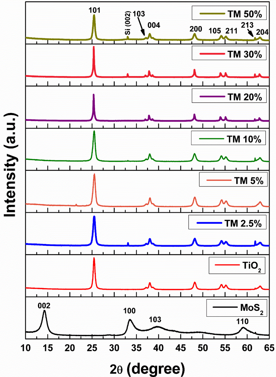
Figure 1. XRD pattern of pure MoS 2 , pure TiO 2 , and MoS 2 /TiO 2 composites with a different weight percentage of MoS 2 .
