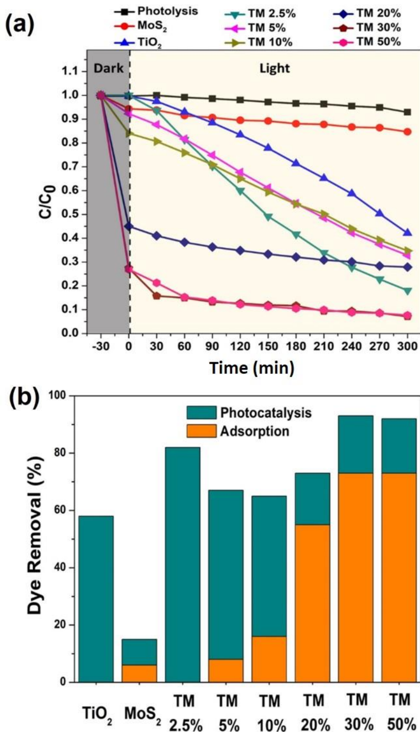
Figure 5. (a) Photocatalytic degradation, (b) dye removal efficiency of MB dye by \text{TiO}_2 , \text{MoS}_2 and \text{MoS}_2/\text{TiO}_2 nanocomposites with a different weight percentage of \text{MoS}_2 . Note that the catalyst loading quantity is 25 mg in 50 ml dye solution.
