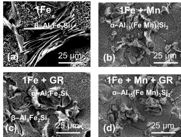
Fig. 5. Deep-etched microstructure (SEM-BSE) illustrating the morphology of \beta - \text{Al}_9\text{Fe}_2\text{Si}_2 and \alpha - \text{Al}_{15}(\text{Fe},\text{Mn})_3\text{Si}_2 IMCs formed in (a) 1 wt.% Fe, (b) 1 wt.% Fe + 0.5 wt.% Mn (Fe: Mn ratio 0.5), (c) Al-5Ti-1B inoculated 1 wt.% Fe, and (d) inoculated 1 wt.% Fe + 0.5 wt.% Mn alloy.
