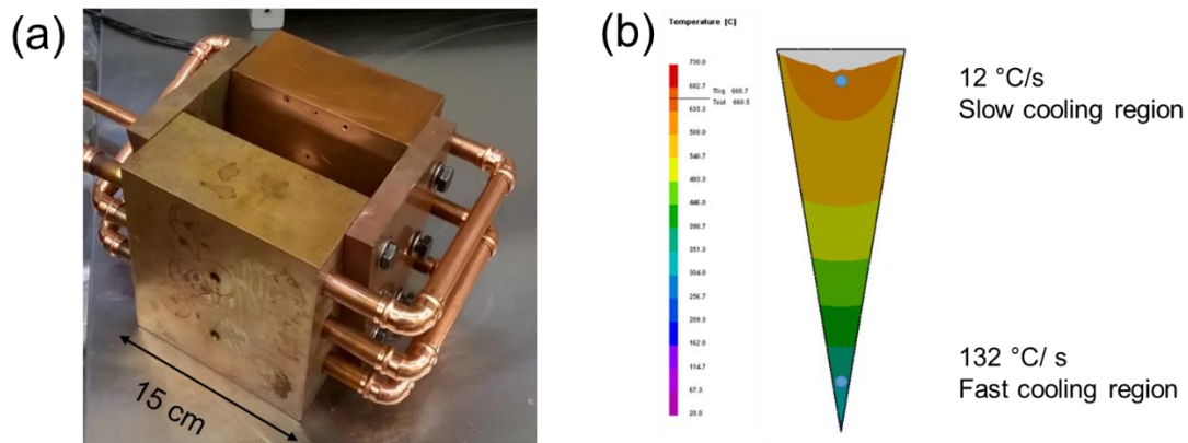
Fig. 1. (a) Copper wedge shape mould and (b) ProCAST simulated cross section showing regions experiencing slow ( 12 °C/s) and fast cooling (132 °C/s), respectively.
