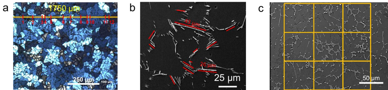
Fig. 2. The statistical analysis methods: (a) the linear intercept method on polarised light micrograph, (b) the line measuring the \beta -(Al 9 Fe 2 Si 2 ) Fe IMCs platelet size, and (c) the quadrant method on low magnified SEM micrograph.
