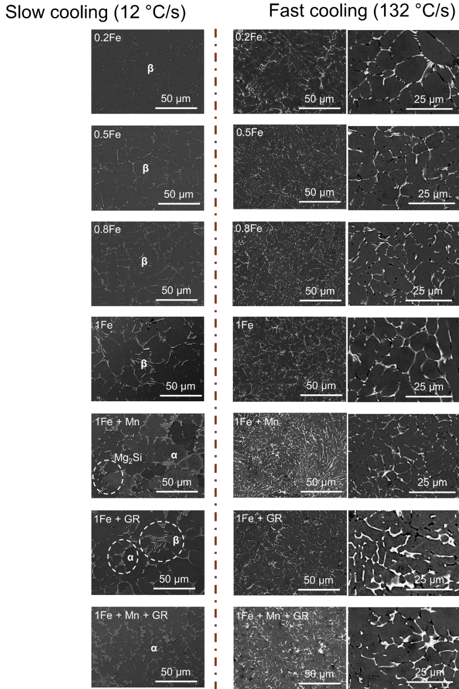
Fig. 4. SEM- BSE images from solidified ingots illustrating the variation in Fe-intermetallic size, distribution and morphologies with the cooling condition, Fe content and inoculant addition.
