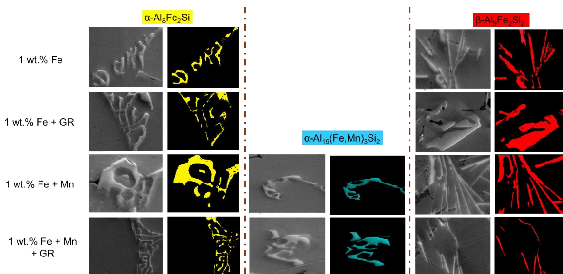
Fig. 7. SEM micrographs and EBSD phase mapping showing the hexagonal \alpha - \text{Al}_8\text{Fe}_2\text{Si} , cubic \alpha - \text{Al}_{15}(\text{Fe},\text{Mn})_3\text{Si}_2 and monoclinic \beta - \text{Al}_9\text{Fe}_2\text{Si}_2 IMC phase in 1.0 wt. % Fe from the slow cooled region (12 ^\circ\text{C/s} ).
