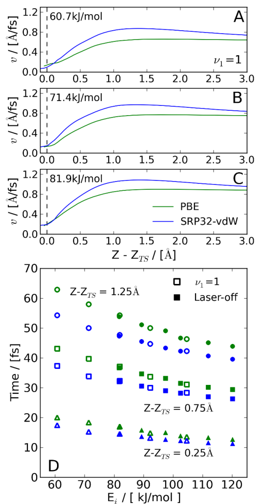
FIG 6. The average velocity of the PBE (green) and SRP32-vdW (blue) trajectories that react as they approach the surface at an incident energy of 60.7 kJ/mol (A), 71.4 kJ/mol (B) and 81.9 kJ/mol (C) with a quantum of initial C-H stretch excitation. The dashed vertical line shows the position of the transition state. Panel D: The average time it takes for the scattered trajectories to travel a distance \Delta Z of 1.25 \text{\AA} (circles), 0.75 \text{\AA} (squares) and 0.25 \text{\AA} (triangles) along Z to Z_{TS} for the PBE trajectories (green) and the SRP32-vdW trajectories (blue). The open symbols show the times for the trajectories prepared with a quantum of C-H stretch, and the filled symbols the laser-off trajectories.
