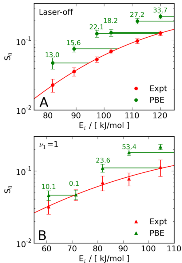
FIG 1. Comparison of the experimentally measured sticking coefficients 39 (red) with those calculated using the PBE functional (green) for \text{CHD}_3 dissociation on Pt(111) under laser-off conditions (A) and for molecules prepared with a single quantum of C-H stretch vibration (B). The numbers in the plots are the energy shift in kJ/mol between S_0 calculated with the PBE functional and the fit to the experimental data.
