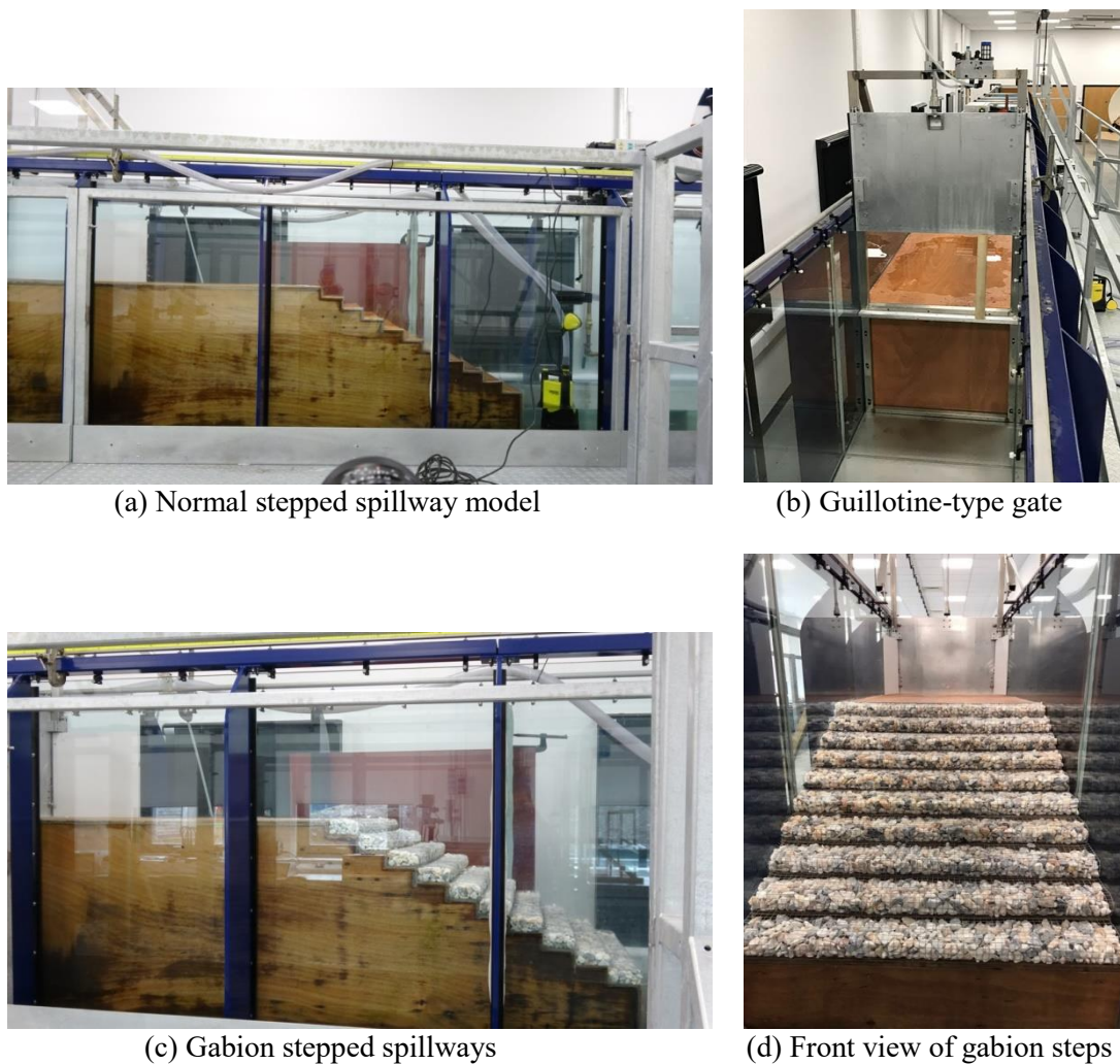
Figure 3. Experiment set-up.
