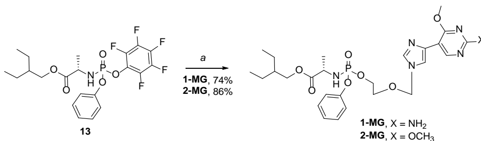
Scheme 3. Reagents and conditions: (a) 1 or 2 , tBuMgCl, THF, rt, overnight.
