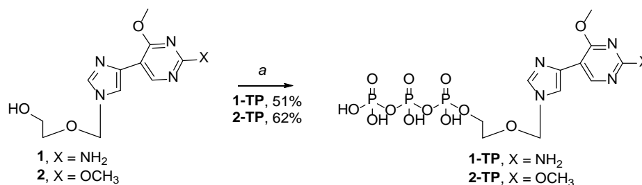
Scheme 4. Reagents and conditions: (a) i. 1 or 2 , SalPCl, Pyr, 1,4-dioxane, rt, 45 min; ii. tributyl ammonium pyrophosphate, tributylamine, DMF, rt, 45 min; iii. I 2 , H 2 O, Pyr, rt, 30 min.
