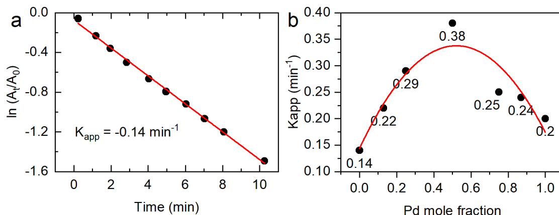
Fig. 6: a) \ln(A_t/A_0) as a function of time (minutes) for the reduction of 4-NP by NaBH 4 over 1wt.% Au/TiO 2 , as a representative example, b) K_{app} (min -1 ) as a function of Pd mole fraction over different Au x Pd 1-x /TiO 2 catalysts. Reaction condition: 4-NP/metal molar ratio= 13, NaBH 4 /4-NP molar ratio = 30, T = 30 °C and stirring rate = 1000 rpm.
