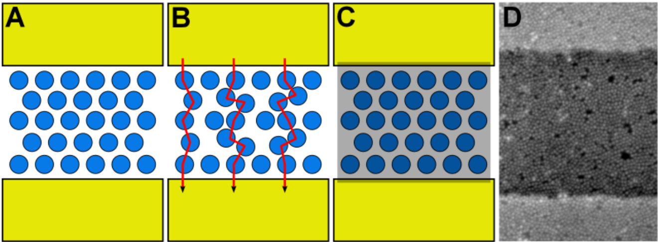
FIG. 1: Possible mechanisms. A) Pristine, well ordered sample, B) first possible conduction mechanism after annealing: shift of nanoparticles and enhanced conductivity through paths with shorter tunnel barriers, C) second mechanism: carbonization of ligands. D) SEM image of a CoPt nanoparticle monolayer deposited on a substrate structured with gold electrodes (the brighter parts).
