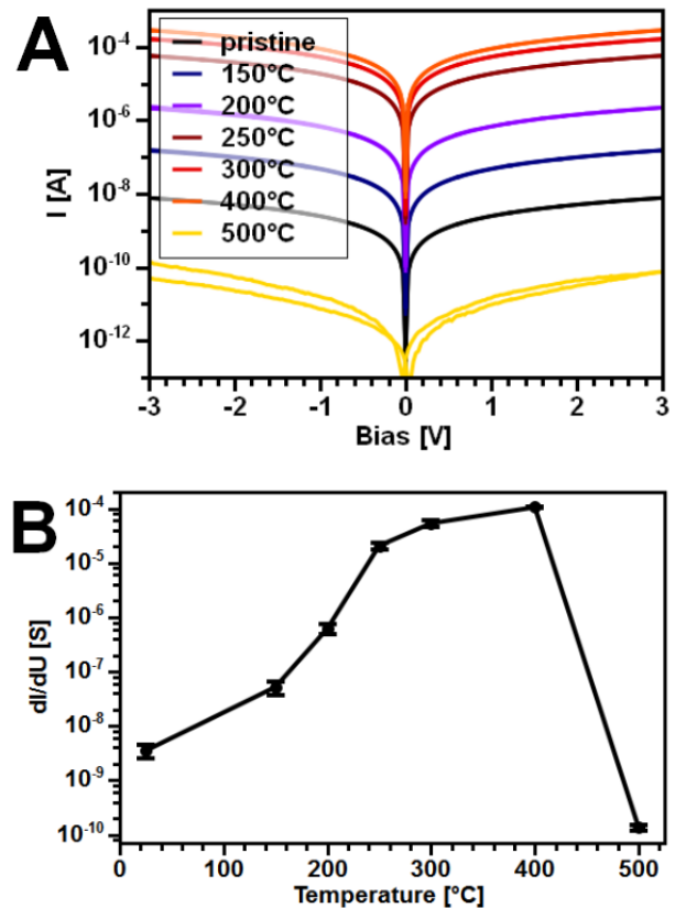
FIG. 2: A) I-V curves of a monolayer film, annealed at different temperatures and measured at room temperature. The conductivity increases with increasing annealing temperature up to 400°C. B) The conductivity at 3 V plotted against the annealing temperature.
