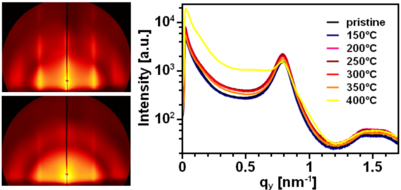
FIG. 4: Left: GISAXS pattern of thermally untreated particle film (upper image) and a film annealed at 400°C (lower image). The structural change is well visible in the loss of clarity of the reflections. Right: curves obtained by slicing the GISAXS pattern along the q_y axis.
