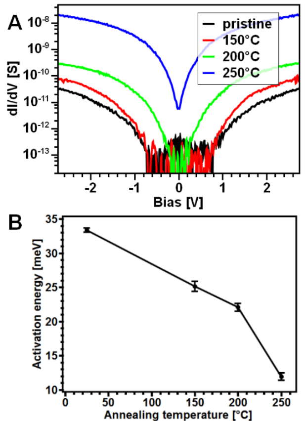
FIG. 6: A) Differential conductance of a pristine and annealed films at 4.3 K. The film annealed at 250^\circ\text{C} shows no sign of Coulomb blockade at 4.3 K and zero bias, while the untreated film clearly shows blockade below half a volt. The film treated at 200^\circ\text{C} shows reduced Coulomb blockade. B) The activation energy decreases with increasing annealing temperature (at 2 V).
