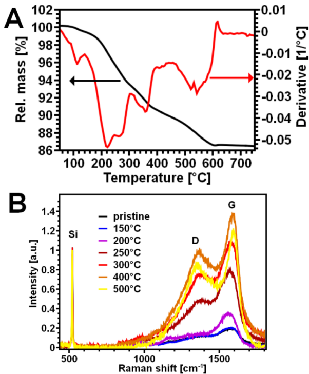
FIG. 5: A) Result of a thermo-gravimetric measurement (black) and the first derivative (red). The measurement was performed under nitrogen flow and with a heating rate of 20^\circ\text{C}/\text{min} . B) Raman spectrum of a film annealed at different temperatures. The graphs are normalized to the silicon peak. The D and G peak intensity increases with rising annealing temperature. The G peak shifts to higher values with increasing annealing temperature.
