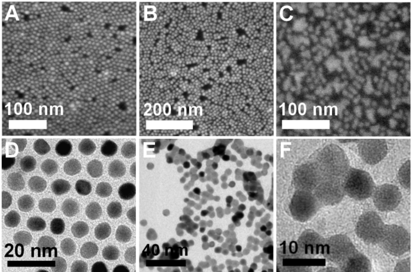
FIG. 3: SEM images of monolayer films A) pristine, B) annealed at 400^{\circ}\text{C} and, C) at 500^{\circ}\text{C} . The annealed films show rifts and agglomerates. D) TEM image of as-synthesized nanoparticles, E) TEM images of particles annealed at 400^{\circ}\text{C} , F) higher magnification.
