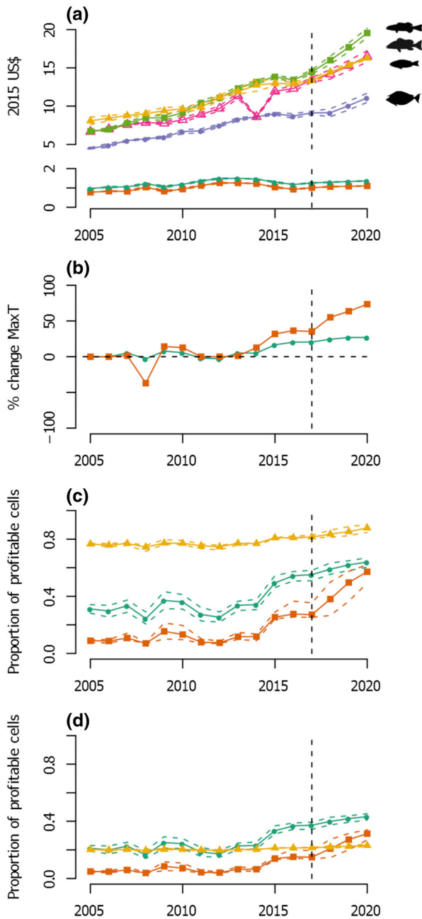
FIGURE 2 Change in fuel costs, fish prices, time to reach profitable reefs, and proportion of profitable reefs of New Caledonia over the time scale of this study (2005–2020). (a) Annual mean price per kilogram of the four main groups of coral reef fish species (from top to bottom: coral trout (squares), snappers and emperors (closed triangles), parrotfish (open triangles), and unicornfish (circles)) and fuel price (green circles—petrol and orange squares—diesel). Shaded areas are 95% confidence intervals of annual means. (b) Percentage change in maximum profitable travel time for each vessel type (size in meters) compared to the 2005 baseline. Orange squares—boats >8 m and green circles—boats >8 m <12 m (boats <5 m not shown). (c) Proportion of profitable accessible reefs for each vessel type across the New-Caledonian archipelago (yellow triangles—boats <5 m). (d) Proportion of all reefs across the New-Caledonian archipelago profitable for each vessel type. Trends to the right of vertical dashed line are predictions post 2017
