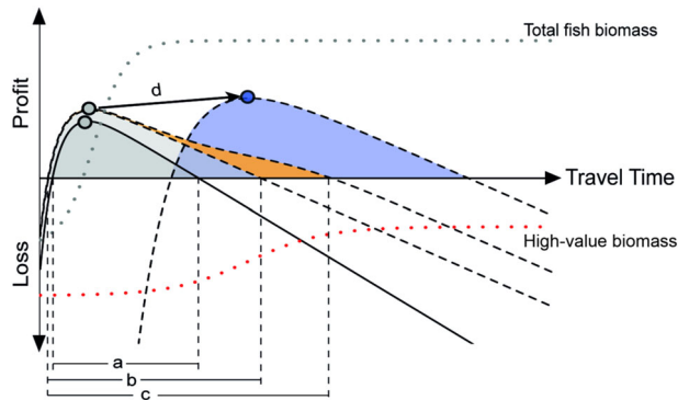
FIGURE 1 Conceptual diagram linking fisheries profitability to travel time from market, fuel cost, and fish price. Black lines are fishery profit–loss curves under low (solid) and high (dashed) fish price scenarios, horizontal line is cost–revenue equilibrium, dotted lines indicate fish biomass, and the gray/blue shaded areas represent profitable fisheries (assuming fixed yield). Gray and blue dots are travel time where profits are maximized for each scenario. Fishing is profitable between a minimum time, where fish become abundant enough to fish, and a maximum beyond which travel becomes too costly (a). If fuel price decreases, or fish price increases, maximum travel time will increase (b). If a high-value species biomass increases with distance from humans at a slower rate than total biomass (red dashed line), decrease in travel costs coupled to increase in fish prices may result in significantly greater maximum travel time, dependent on the rate of increase of the high-value species (c). Similarly, fishery specialization to high-value species will increase both maximum profitable travel time and profits (d)
