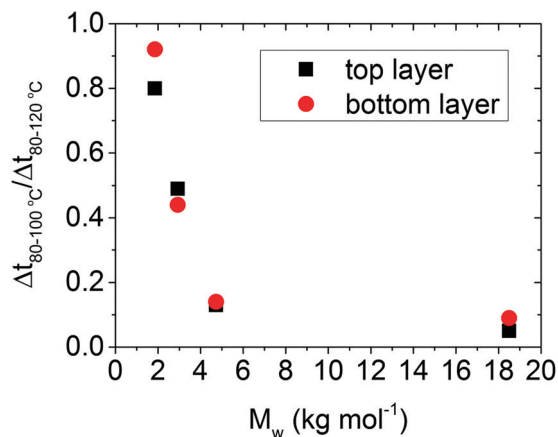
Fig. 4 The ratio of the magnitude of the change in the thickness between 80 °C and 100 °C, \Delta t_{80-100^\circ\text{C}} , to the magnitude of the change in thickness between 80 °C and 120 °C, \Delta t_{80-120^\circ\text{C}} , versus weight-average molecular weight ( M_w ), for the top and bottom layers in each bilayer.
