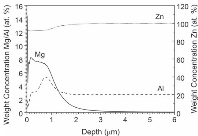
Figure 4. A GDOES depth profile derived from a ZM surface produced by the thermal inter-diffusion of a Mg layer.
