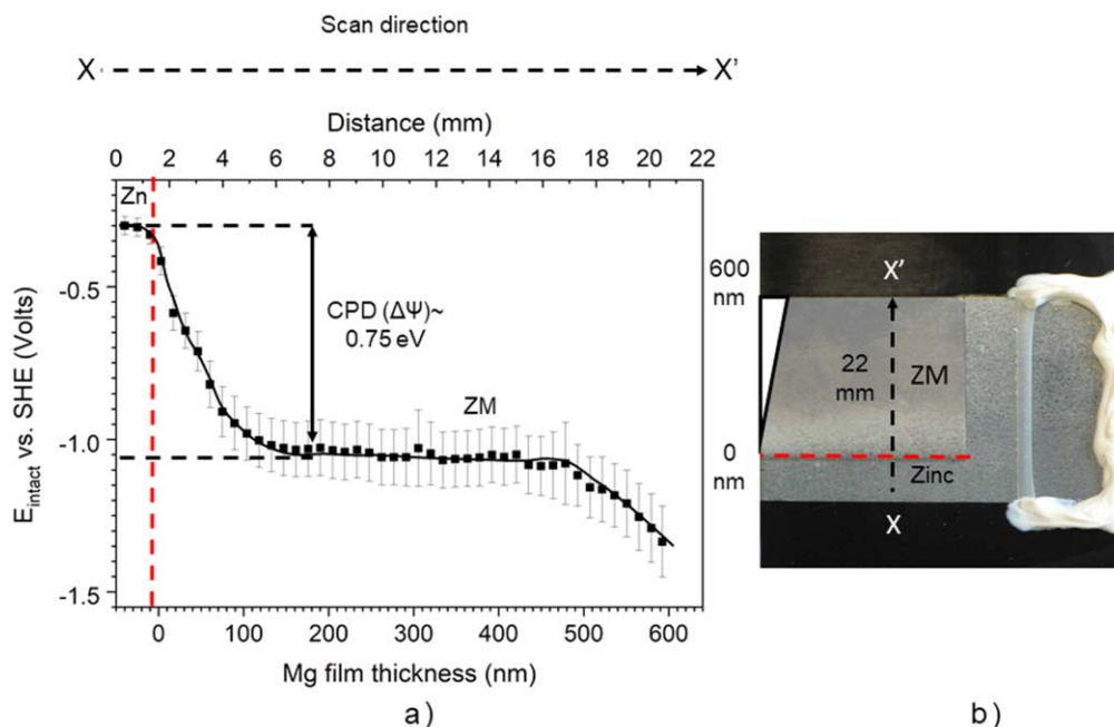
Figure 6. SKP derived E_{intact} values as a function of pre inter-diffusion Mg layer thickness for a PVB coated 600 nm PVD ZM wedge.
