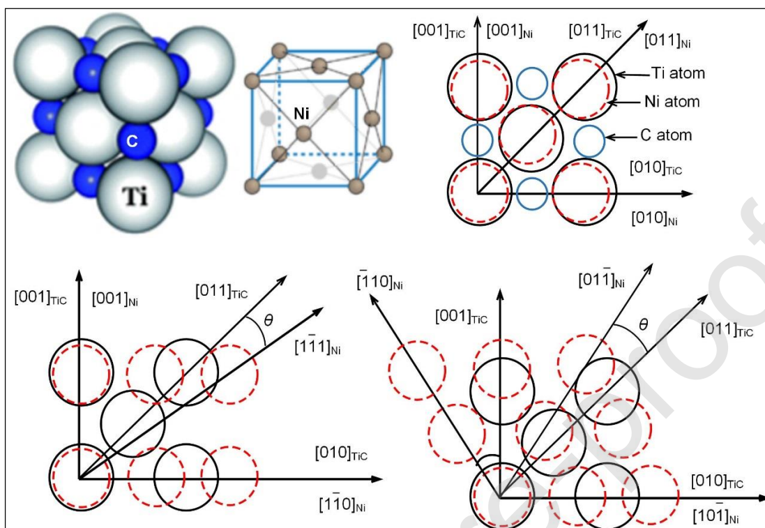
Fig. 2. Schematic representation of lattice disregistry between the face centre cubic (FCC) Ni and TiC crystal structures. This representation is based on Turnbull-Vonnegut and planar crystallographic disregistry theories.
