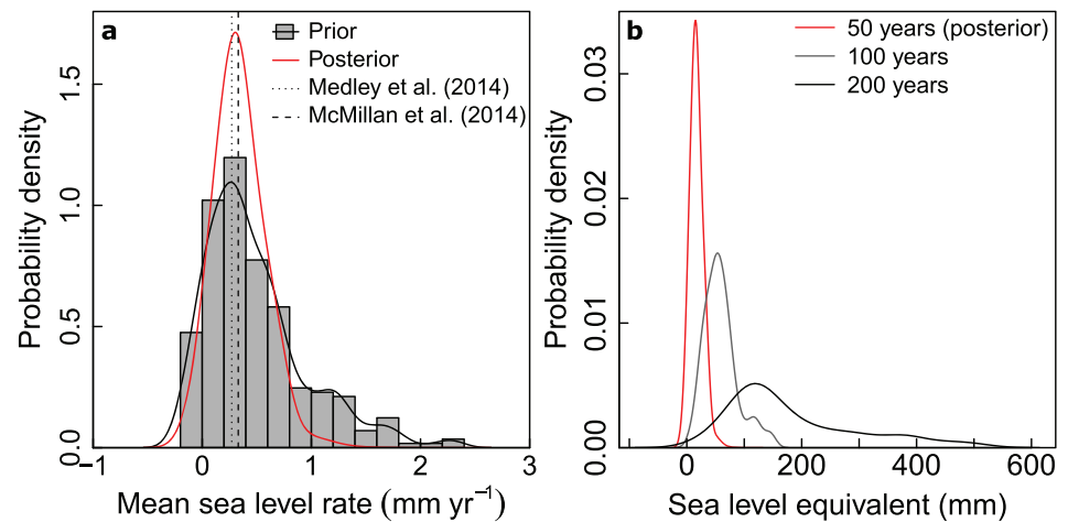
Figure 1. Distributions of sea level change. (a) Histogram (gray boxes) and associated prior probability density function (prior PDF, black curve) of present-day sea-level contribution rate (50-year mean) from the original model ensemble and calibrated posterior PDF (red curve). Observed rates from 2010 using the input-output method ( 0.27 \pm 0.04 mm/year, short dashes; Medley et al. 2014) and 2010–2013 derived from Cryosat-2 altimetry ( 0.33 \pm 0.05 mm/year, long dashes; McMillan et al. 2014) are represented by vertical lines. (b) PDFs of the total sea level contribution from the calibrated 50-year ensemble (red curve) and from the extended ensemble after 100 years (gray curve) and 200 years (black curve).
