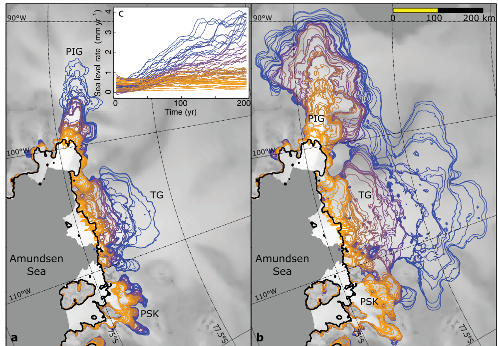
Figure 2. Grounding line position after (a) 100 years and (b) 200 years. Each colored line represents an individual ensemble member: yellow represents a more linear sea level response and blue represents a super-linear response (based on the second derivative of the sea level trend shown in [c] the 8-year running mean of the rate of sea level contribution from the ASE during the 200-year simulations). The initial grounding line position is delineated by the thick black line. Gray scale background indicates initial velocity.
