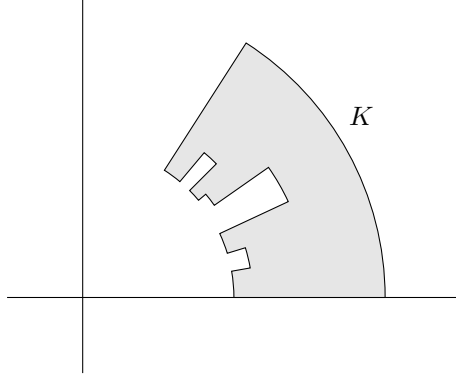
FIGURE 1. The construction of the set K \subseteq \mathbb{R}^2 in the proof of Theorem 4.22: here I_0, I_3 \subseteq [0, 1] \setminus A overlap.
