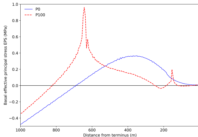
Figure 10. Comparison of basal stresses using the Coulomb sliding law with partial hydraulic connectivity at the ice–bed interface, before (P0) and after (P100) cutting of a 100 m notch. Ungrounding occurred between approximately 160 and 640 m for P100 and not at all for P0.
