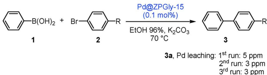
Scheme 1. Representative Suzuki–Miyaura coupling catalysed by Pd nanoparticles supported on Zr_2(PO_4)H_5(O_3PCH_2)_2NCH_2COO]_2 \cdot H_2O nanosheets (15 wt. % Pd). Reprinted with permission from ref. [108]. Copyright 2015, Royal Society of Chemistry.
