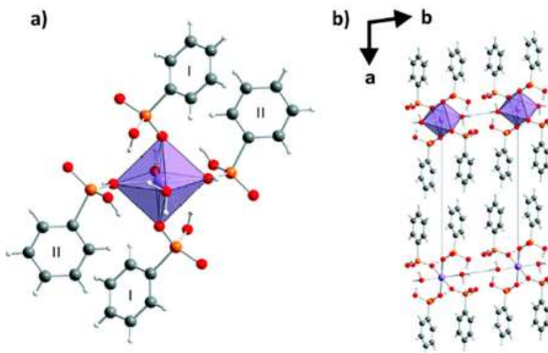
Figure 10. Crystal structure of [\text{Mn}(\text{HO}_3\text{PPh})_2-(\text{H}_2\text{O}_3\text{PPh})_2(\text{H}_2\text{O})_2] ( 1 ), with respective values for the isomorphous compounds based on \text{Co} ( 2 ) and \text{Ni} ( 3 ). (a) Coordination sphere of the metal ion. (b) Structure of 1 shown along the c -axis (b). Hydrogen atoms are omitted for clarity. Colour code: purple: manganese, red: oxygen, orange: phosphorus, grey: carbon, light grey: hydrogen. Adapted with permission from reference. [57]. Copyright 2016, Royal Society of Chemistry.
