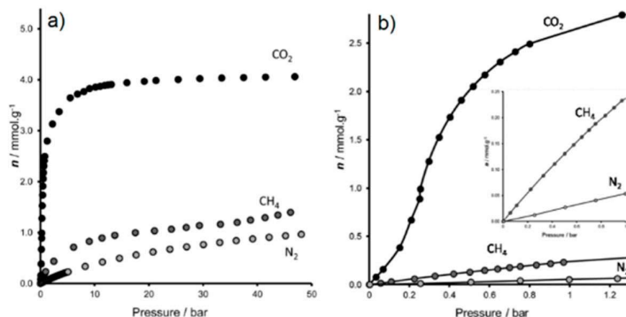
Figure 26. CO 2 , CH 4 , and N 2 adsorption isotherms measured at 303 K on MIL-91(Al) up to 50 bar (left) and up to 1 bar (right). Adapted with permission from reference. [69]. Copyright 2015, American Chemical Society.
