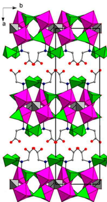
Figure 22. Crystal structure of Zr_2(PO_4)H_5[(O_3PCH_2)_2NCH_2COO]_2 \cdot H_2O viewed along the c -axis. Colour code: zirconium: pink, phosphorus: green, oxygen: red, nitrogen: blue, carbon: grey. Reprinted with permission from reference. [107]. Copyright 2014, American Chemical Society.
