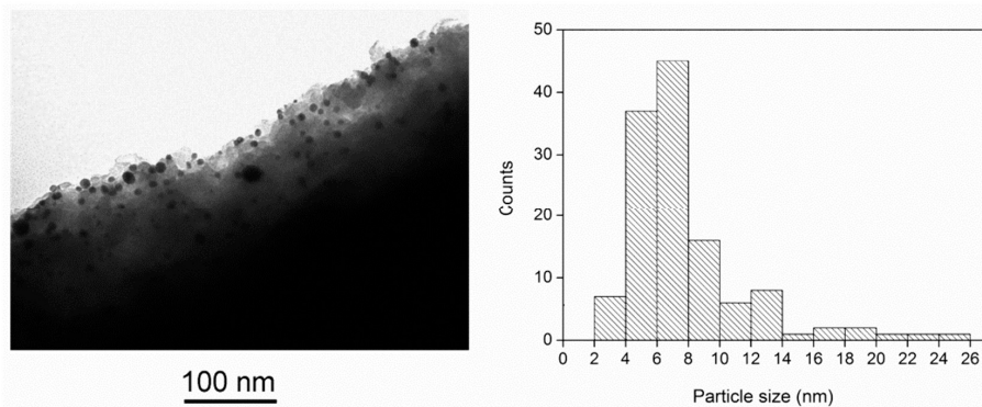
Figure 24. Transmission electron micrograph of Au@ZP-AEP (left) and Au particle size distribution (right). Adapted with permission from reference [111]. Copyright 2019, Royal Society of Chemistry.
