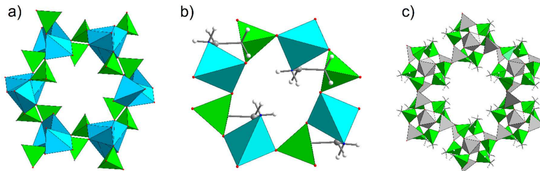
Figure 5. Crystal structures of the open framework metal phosphonates (MPs): (a) \beta\text{-Cu}(\text{CH}_3\text{PO}_3)_2 , (b) \text{Zn}(\text{O}_3\text{PC}_2\text{H}_4\text{NH}_2) , and (c) \alpha\text{-Al}_2(\text{O}_3\text{PCH}_3)_2 . Colour code: light blue: copper, turquoise: zinc, light grey: aluminium, green: phosphorus, red: oxygen, blue: nitrogen, grey: carbon, white: hydrogen.
