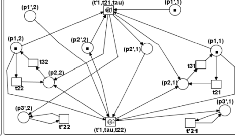
Fig. 6. Synchronous firing transitions and arcs Fig. 7. Result of transforming ERS
