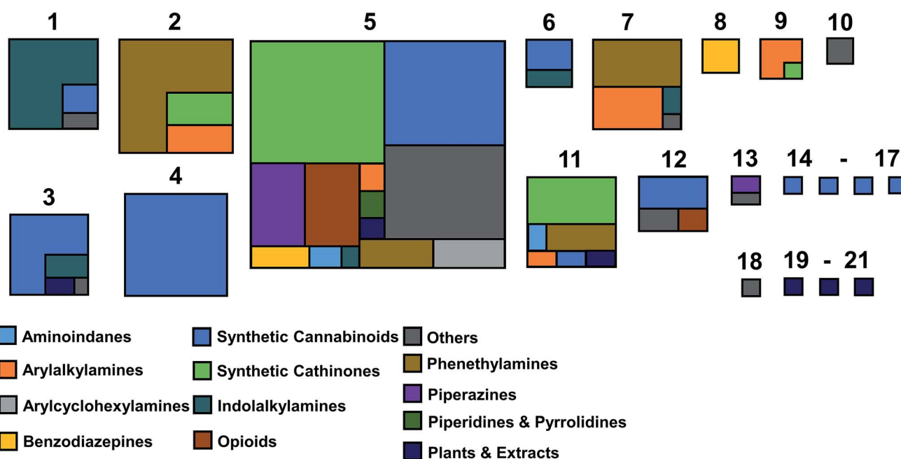
Fig. 4 Illustration of the proportion of compounds according to the EMCDDA/EDND NPS categories found in each of the dendrogram's superclusters. The relative size of each box is proportional to the number of compounds contained in the supercluster.
