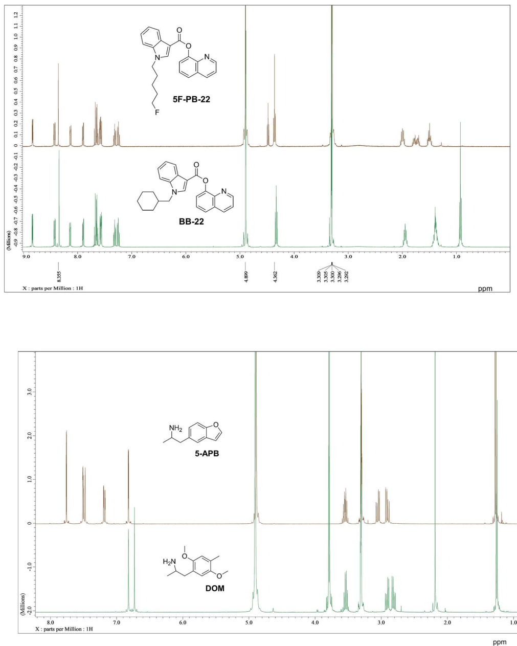
Fig. 7 1\text{D } ^1\text{H} NMR spectra of representative NPS (green) and the members of their respective clusters (brown). Full spectral range for 5-APB and DOM available in ESI.†
