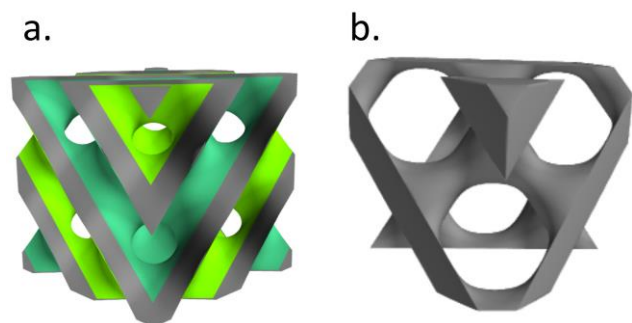
Figure 1. (a) Q_{II}^D 'double diamond' phase where grey region is occupied by lipid bilayer, (b) corresponding 'single diamond' platinum structure.
