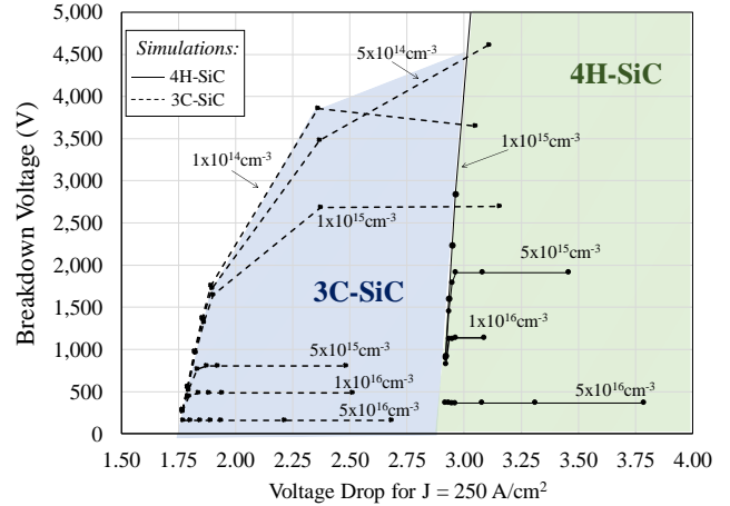
Fig. 9. Breakdown voltage of 3C-SiC and 4H-SiC P-i-N PT power diodes as a function of voltage drop at 250\text{A}/\text{cm}^2 . The equi-doping lines resemble a constant doping concentration for various values of increasing thickness, displayed as filled cycles, beginning from the left most side towards the right most side of each line.
