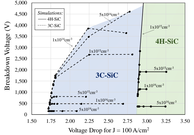
Fig. 8. Breakdown voltage of 3C-SiC and 4H-SiC P-i-N PT power diodes as a function of voltage drop at 100\text{A}/\text{cm}^2 . The equi-doping lines resemble a constant doping concentration for various values of increasing thickness, displayed as filled cycles, beginning from the left most side towards the right most side of each line.
