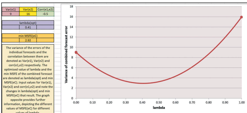
Figure 1. Forecast combination.
