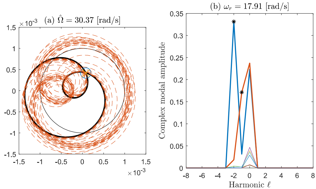
Figure 15: An unstable orbit at \Omega=30.4 rad/s. (a) Solid black line shows orbit predicted by normal forms analysis, orange dashed line shows time simulation. Marker shows initial point for both orbits. (b) Amplitude of complex modal components of analytical solution; thick lines show resonant modes and asterisk markers show resonant harmonics of those modes.
