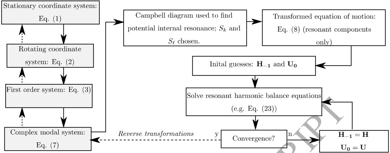
Figure 1: Summary of the normal forms solution process.
