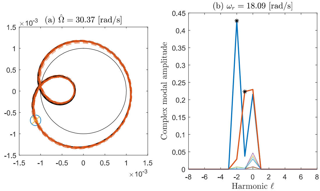
Figure 14: A stable orbit at \Omega=30.4 rad/s, showing trace of the shaft centrepoint. (a) Solid black line (obscured) shows orbit predicted by normal forms analysis, orange dashed line shows time simulation. Marker shows initial point for both orbits. (b) Amplitude of complex modal components of analytical solution; thick lines show resonant modes and asterisk markers show resonant harmonics of those modes.
