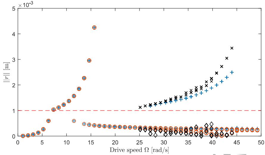
Figure 13: Normal forms results compared to brute force bifurcation. + show max r from simulation, \circ shows minimum results. Crosses \times show the maximum r from analysis, diamonds show the minimum r from analysis. (Non-contacting results from analysis are omitted)
