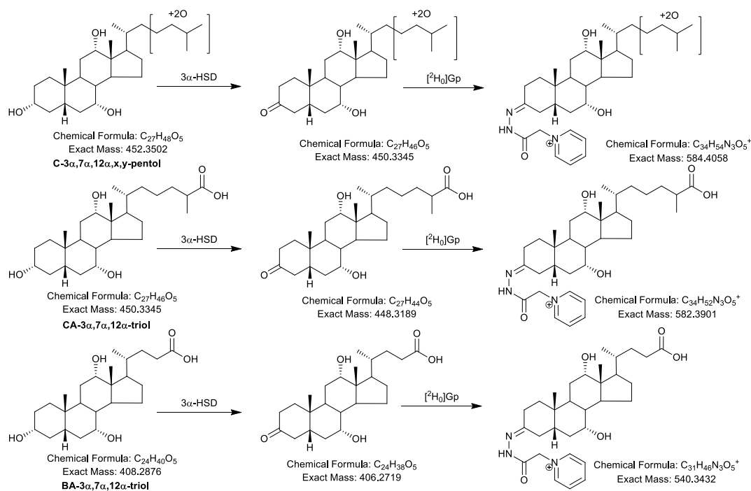
Scheme 2. Structures of bile alcohols and acids, and their products of 3α-HSD oxidation and GP-derivatization.
