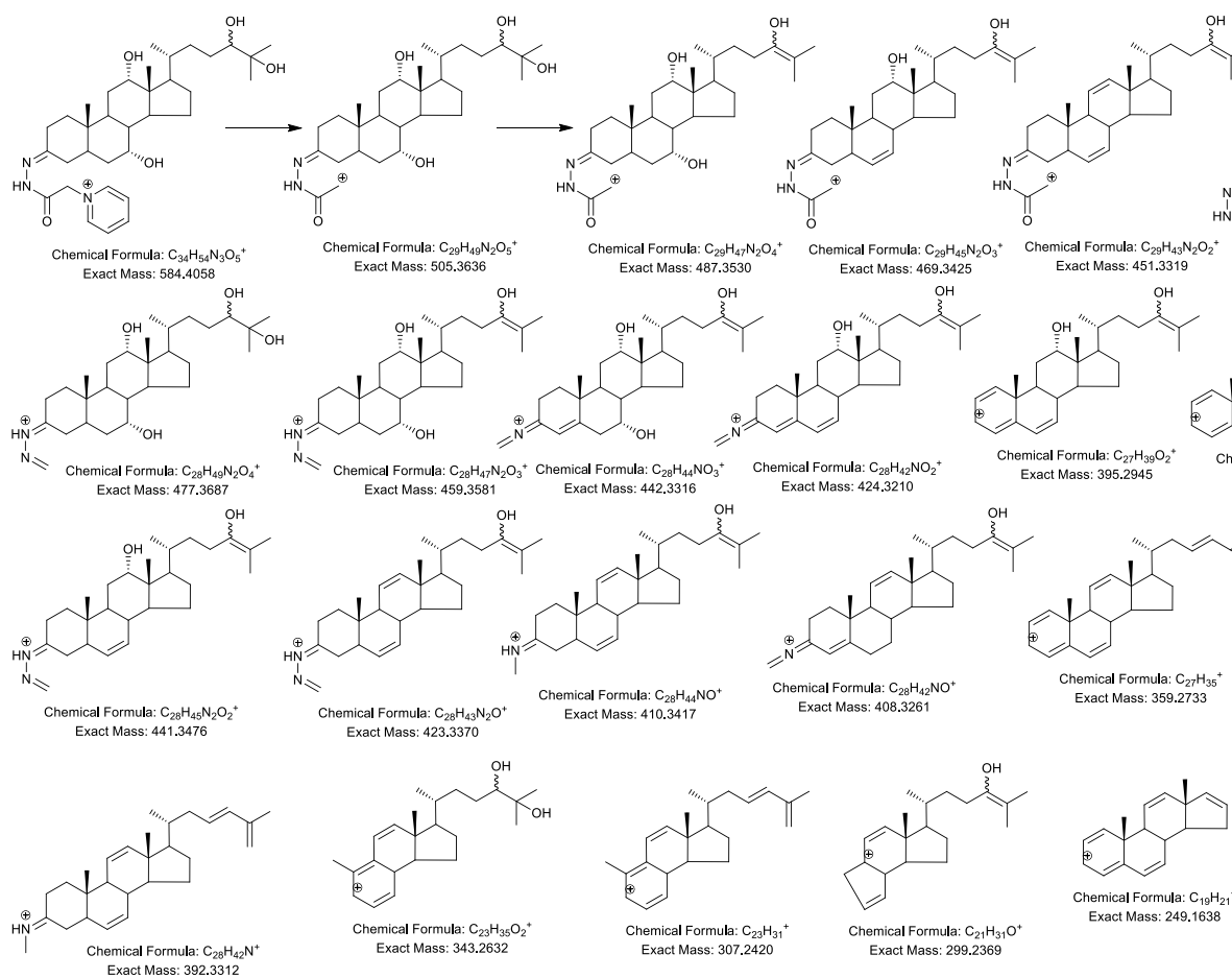
Scheme 4. MS 2 and MS 3 fragmentation of oxidized/GP-derivatized pentahydroxy-bile alcohols as illustrated by C-3 \alpha ,7 \alpha ,12 \alpha ,24-hydroxy-24-ene structure are likely to rearrange to the 24-ketone. For simplicity the fragmented Girard derivatizing group is shown as a phenyl ring. Cyclic isomers are similar to those depicted in Scheme 1. See Supplemental Schemes S5–S7 for fragmentation schemes of other
