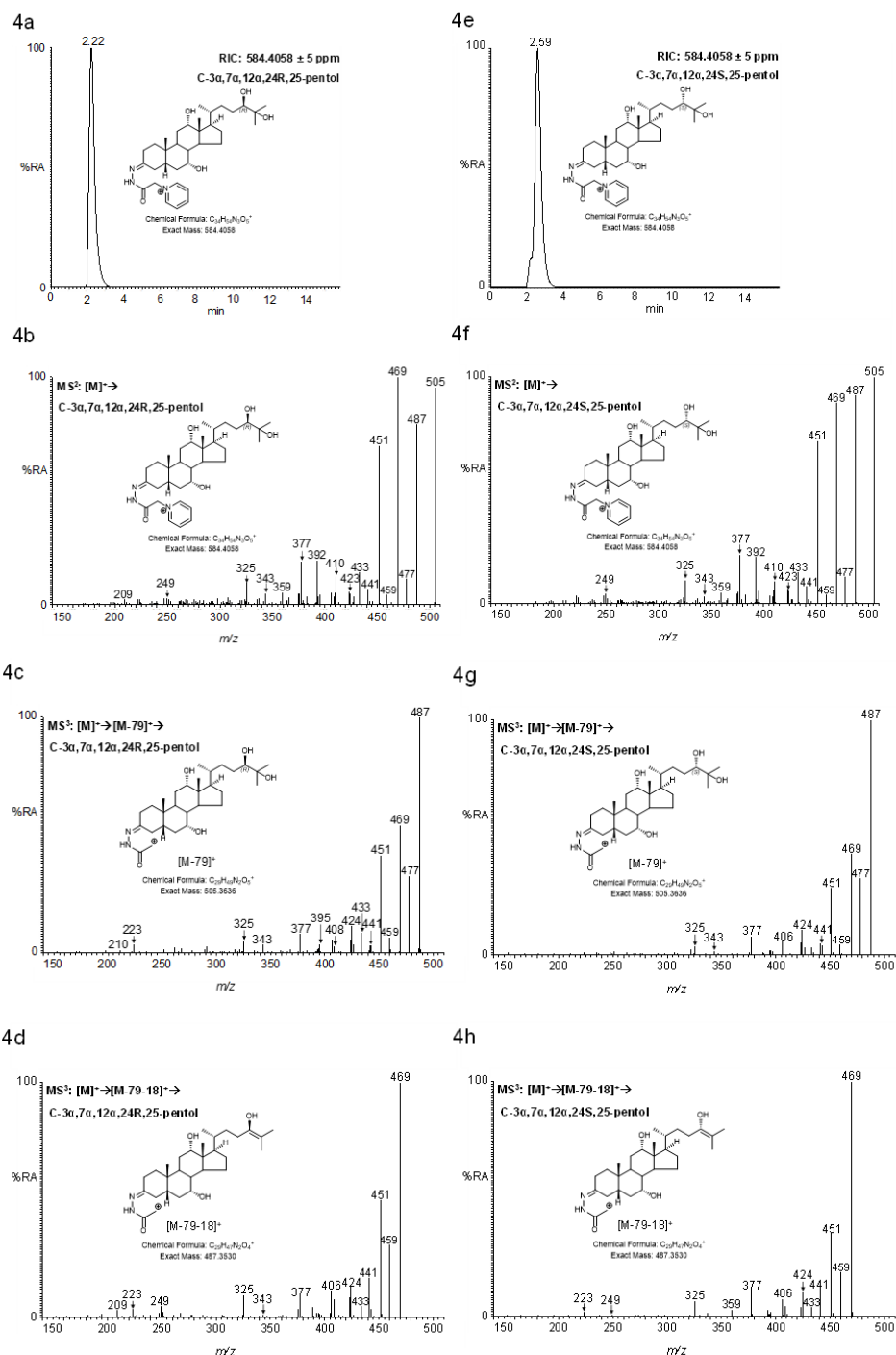
Figure 4. LC-(MS)MS n analysis of oxidized/GP-derivatized C-3 \alpha ,7 \alpha ,12 \alpha ,24R,25-pentol and C-3 \alpha ,7 \alpha ,12 \alpha ,24S,25-pentol: (a) RIC, (b) MS 2 ([M] + →), (c) MS 3 ([M] + → [M-Py] + →), and (d) ([M] + → [M-Py-18] + →) from the analysis of C-3 \alpha ,7 \alpha ,12 \alpha ,24R,25-pentol. (e) RIC, (f) MS 2 ([M] + →), (g) MS 3 ([M] + → [M-Py] + →), and (h) ([M] + → [M-Py-18] + →) from the analysis of C-3 \alpha ,7 \alpha ,12 \alpha ,24S,25-pentol. Data was generated on the Orbitrap-Elite mass spectrometer as in Figure 1. Fragment ions are described in Table 1 and postulated structures are shown in Scheme 4.
