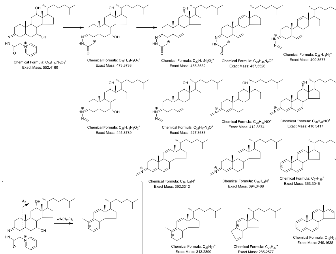
Scheme 3. MS 2 and MS 3 fragmentation of oxidized/GP derivatized bile alcohols as illustrated by C-3 \alpha ,7 \alpha ,12 \alpha -triol. For simplicity, the GP group is shown in its linear isomeric form. The inset shows fragmentation route A 3 leading to the [A 3 -H-(H 2 O) 2 ] + fragment. See Supplemental Schemes S1–S4 for fragmentation schemes of other trihydroxy- and tetrahydroxy-bile alcohols and their corresponding m/z with fragment ion composition.
