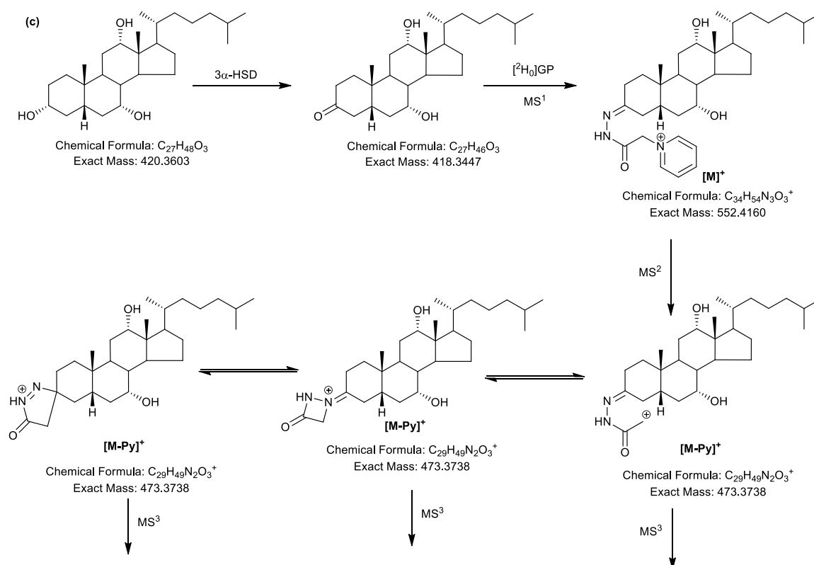
Scheme 1. Enzyme-assisted derivatization for sterol analysis (EASDA): (a) EADSA of the 3\beta -hydroxy-5-ene function using cholesterol oxidase and [^2H_5] Girard P reagent ( [^2H_5]GP ); (b) derivatization of the 3-oxo-4-ene function with [^2H_0]GP ; (c) EADSA of the 3\alpha -hydroxy-5 \beta -hydrogen function with 3\alpha -hydroxysteroid dehydrogenase ( 3\alpha -HSD) and [^2H_0]GP . Derivatives with the [^2H_5]GP and [^2H_0]GP reagents can be combined and analyzed in a single LC-MS run. Other isotope-coded GP reagents have been synthesized to allow triplex analysis if required [45].
