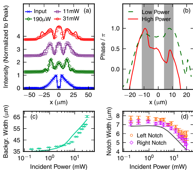
FIG. 3. As Fig. 2 for the amplitude defect initial condition.
