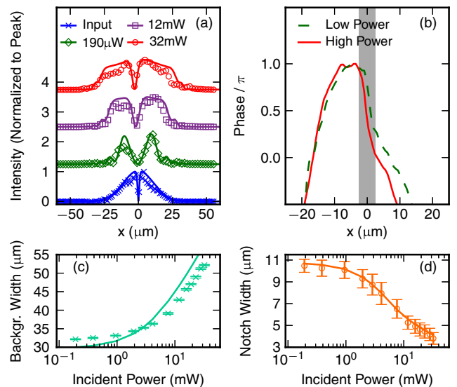
FIG. 2. Dark-soliton formation from the phase jump initial condition. (a) Experimental (points) and theoretical (full lines) intensity profiles of input field and output fields at three powers. (b) Experimental output phase at low and high power. [(c) and (d)] Experimental (points) and theoretical (full lines) power dependences of full width at one third maximum of background and FWHM of dark notches.
