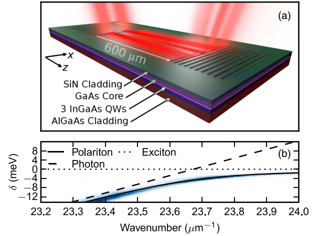
FIG. 1. (a) Schematic of polariton waveguide, and (b) lower polariton dispersion relation seen in the angle resolved photoluminescence spectrum.
