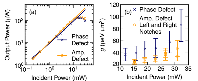
FIG. 4. (a) Output vs incident power for the two initial conditions. (b) Nonlinearity deduced from soliton width.
