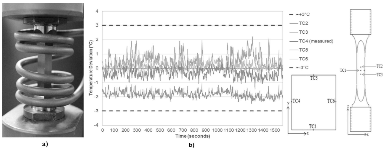
Fig. 10. (a) Non-uniform multi-turn longitudinal field helical coil (b) Temperature distribution associated with non-uniform multi-turn longitudinal field helical coil, showing a spread of +/-3°C in temperature across the critical volume of material around the crack.
