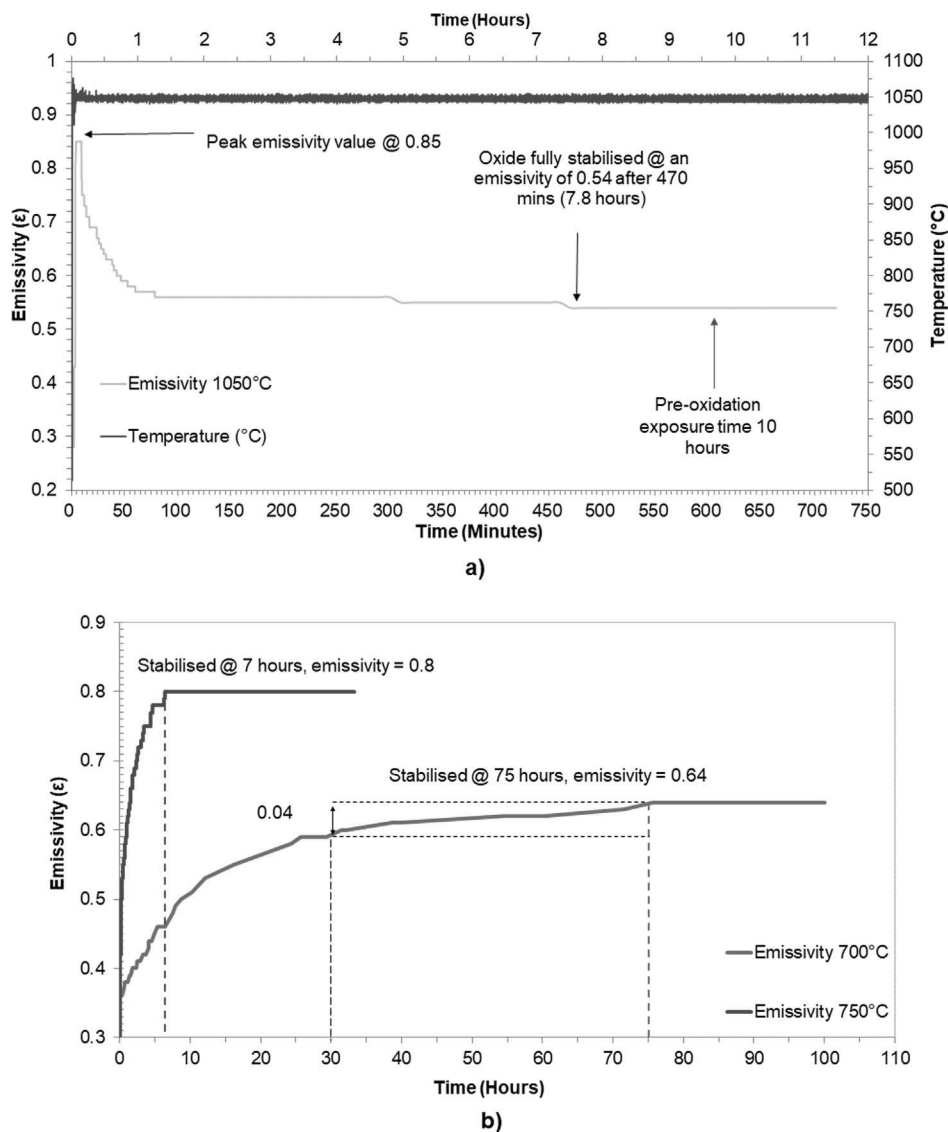
Fig. 1. Emissivity profile of (a) CMSX-4, showing the oxide stabilised at an emissivity of 0.54 after 7.8 h at 1050 °C and (b) RR1000, showing the oxide stabilised at an emissivity of 0.8 after 7 h at 750 °C and at an emissivity of 0.64 after 75 h at 700 °C.
