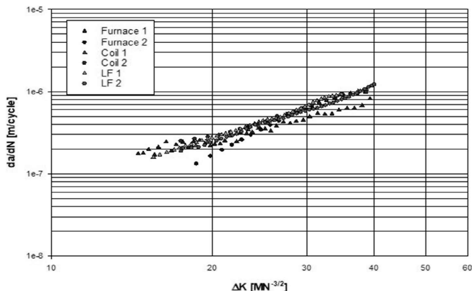
Fig. 13. Graph comparing da/dN vs \Delta K of Ti-6246 corner crack specimens tested at the same isothermal conditions, using three different heating methods – ICS, radiant lamp furnace and conventional furnace. Crack growth rates are consistent across heating methods.
