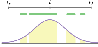
Fig. 6. Node (edge) transparency when aggregating a small multiple across time. We consider a Gaussian curve centred at t and with standard deviation equal to a sixth of the cluster interval in time. The appearance of the graph element in time is extracted (green lines). The transparency of the element is the area under the Gaussian during the appearance intervals (yellow) divided by the total area under the curve.
