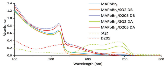
Fig. 2 Absorption spectra of control MAPbBr 3 devices, MAPbBr 3 devices co-sensitized with SQ2 and D205 using the DB method (MAPbBr 3 /SQ2 DB and MAPbBr 3 /D205 DB, respectively) and MAPbBr 3 devices co-sensitized with SQ2 and D205 using the DA method (MAPbBr 3 /SQ2 DA and MAPbBr 3 /D205 DA, respectively). The dashed lines represent solid state dyed films of D205 and SQ2.
