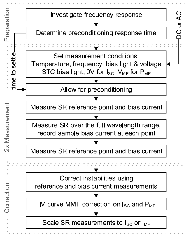
Fig. 7. Proposed universally applicable SR measurement and correction routine; the methodology presented was developed with instabilities of perovskite devices in mind.
