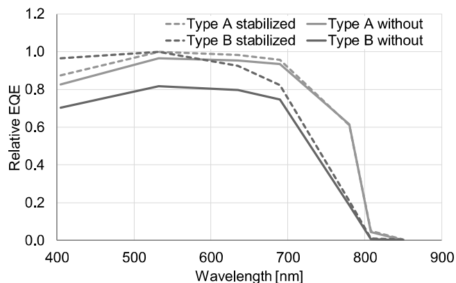
Fig. 2. Measurement error caused during scanning of the EQE curve without allowing the device to stabilize to its bias conditions.
