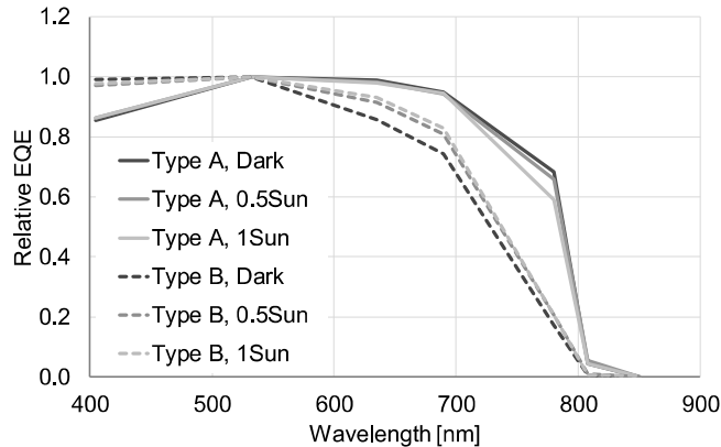
Fig. 5. Relative EQE at different bias irradiance conditions after 10 min preconditioning; both device types show a wavelength-dependent bias light response with opposite trends.
