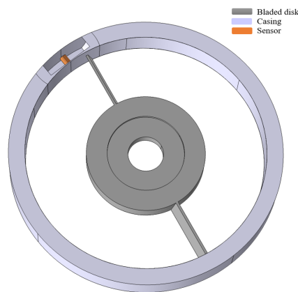
Figure 3: Model geometry of the P-ECS case
