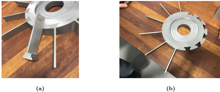
Figure 10: (a) Manufactured blade (b) Manufactured disk
