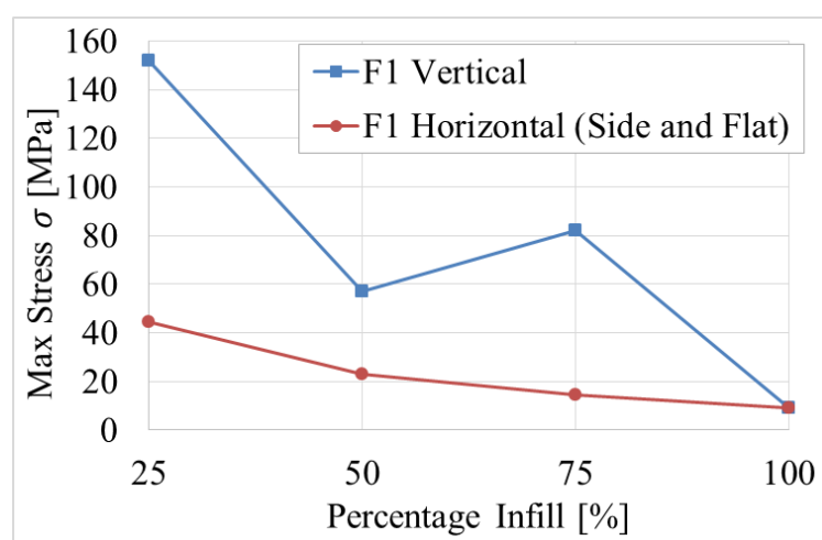
Figure 15. Max stress recorded from Axial Loading (F1).
