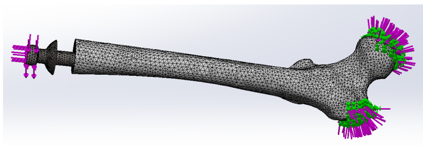
Figure 4. Initial design with mesh control and all force caseloads [11,12].
