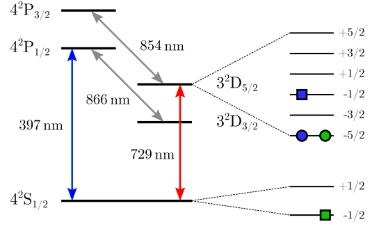
Figure 4: Level scheme of ^{40}\text{Ca}^+ . The green and blue squares and circles indicate different qubit encodings, denoted A and B , respectively. Squares are marking the qubit state |1\rangle whereas the state |0\rangle is highlighted with circles. The corresponding frequency shifts of the transitions caused by the magnetic field are -2.80 MHz/G and +3.36 MHz/G for the qubits marked with green and blue symbols respectively. For configuration 1 described in the enumeration in the main text for both qubits the encoding marked in green is used. The asymmetry in scenario 2 is introduced by encoding one of the qubits in the states illustrated in blue. For the third configuration both qubits again use the encoding marked in green and the spontaneous decay from |0\rangle to |1\rangle is enhanced.
