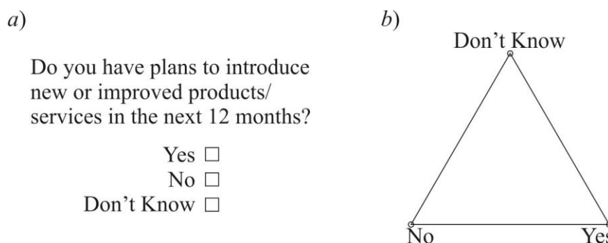
Figure 2. Intended innovation question with response options (a) and response representation in simplex plot domain (b)
