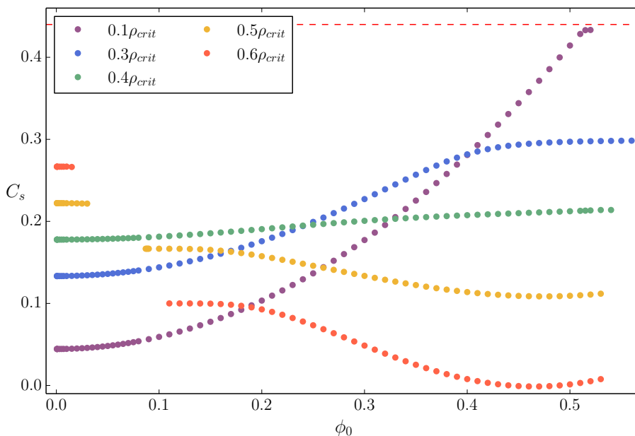
Figure 3. Compactness of constant density objects for \beta = 1 and different values of \phi_0 . The dashed line shows the GR limit for the compactness, which is obtained only for an object with the critical density \rho_{\text{crit}} . The density of each solution is indicated by the point colour. The gap in the sequence of solutions with \rho_0 = 0.5\rho_{\text{crit}} and \rho_0 = 0.6\rho_{\text{crit}} is an effect of the scalar field contributions, as explained in the main text.
