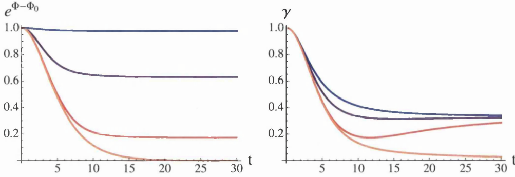
Figure 6.4: On the left are plots of the function e^{\Phi - \Phi_0} for different values of c . On the right, plots of the function \gamma . The orange plots correspond to the minimum value c = 0.125 , the red ones to c = 0.126 , the purple ones to c = 0.15 and the blue ones to c = 0.5 . In the Maldacena-Nastase solution at infinity, there is a linear dilaton and the H_{(3)} vanishes.
