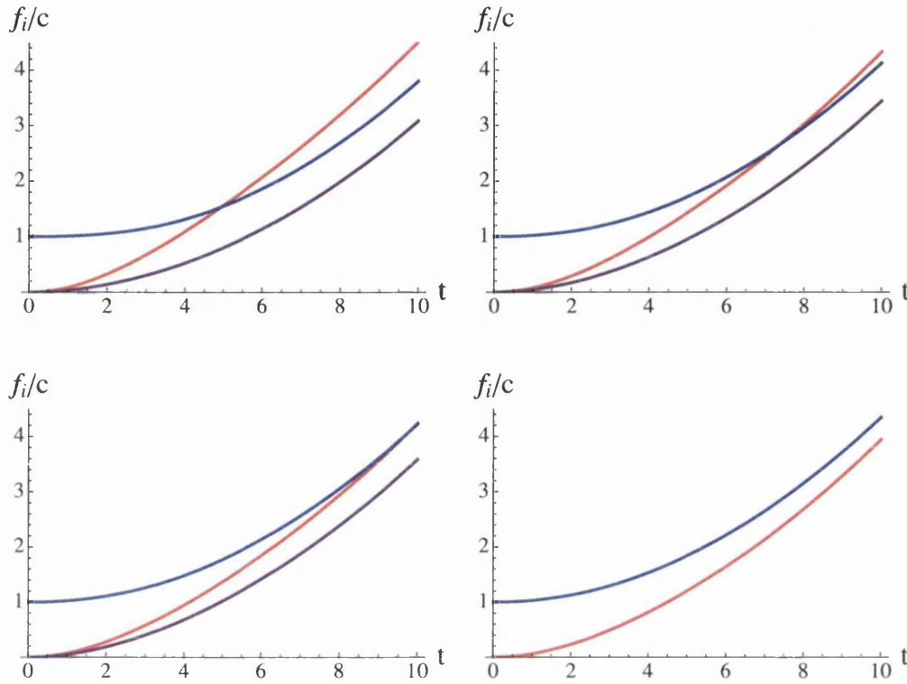
Figure 6.2: Plots of the functions c^{-1} f_i for the X_{31} solution for different values of c . f_1 is in red, f_2 in purple and f_3 in blue. The factor c^{-1} is there for normalisation purposes. From the top left to the bottom right, the values of c are increasing and are 0.2, 0.3, 0.4 for the first three. The bottom-right plot corresponds to the space X_3 where f_1 = f_2 . This is formally the plot for c \rightarrow \infty .
