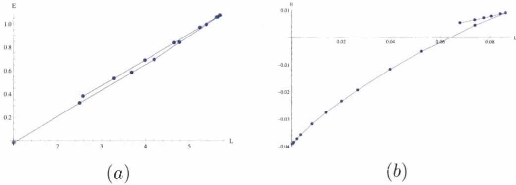
Figure 4.5: Both plots are of E vs. L for a Wilson loop. The plot in (a) corresponds to the class I of UV asymptotics, while the one in (b) corresponds to the UV of class II; both are for \tilde{N}_c = 2 and \tilde{N}_f = 1 .
