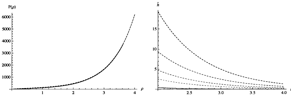
Figure 5.5: On the left: plots of P(\rho) for fixed values c = 30 , \tilde{N}_c = 10 and different values of \tilde{N}_f (and h_1 ). The continuous curve is \tilde{N}_f = 0 . Superimposed on this are the curves for the following values: \tilde{N}_f = 5 (dotted green), \tilde{N}_f = 10 (dotted red), \tilde{N}_f = 20 , (dotted blue), \tilde{N}_f = 40 (dotted black). On the right: different plots of \hat{h}(\rho) for the same values of \tilde{N}_f .
