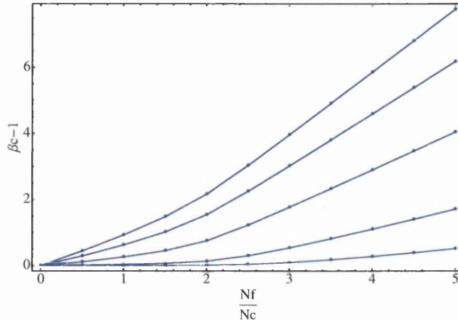
Figure 7.3: We plot the different values of \beta_c - 1 as one varies the ratio N_f/N_c . The curves are for fixed width \delta = 0.2 but different quark masses: moving from the upper curve to the lower one, the values used are r_0 = 0, 0.15, 0.3, 0.7, 1.2 . Notice that, as r_0 increases (the mass increases), the growth of \beta_c with N_f/N_c is less and less noticeable, and the solution in the unflavoured region is almost that of [13] ( \beta_c \simeq 1 ). This was to be expected since the more massive the flavours are, the less they affect the IR dynamics.
