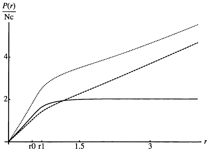
Figure 7.2: Numerical solutions for N_c^{-1}P for different values of N_f/N_c , keeping fixed the profile (flat measure), r_0 and \delta (in the plot, \cosh(4r_1) = \cosh(4r_0) + \delta ). The blue dotted line corresponds to N_f/N_c = 1 . The purple line corresponds to the conformal case N_f/N_c = 2 . And the olive dotted line corresponds to N_f/N_c = 3 . Notice the expected asymptotic UV behaviour.
