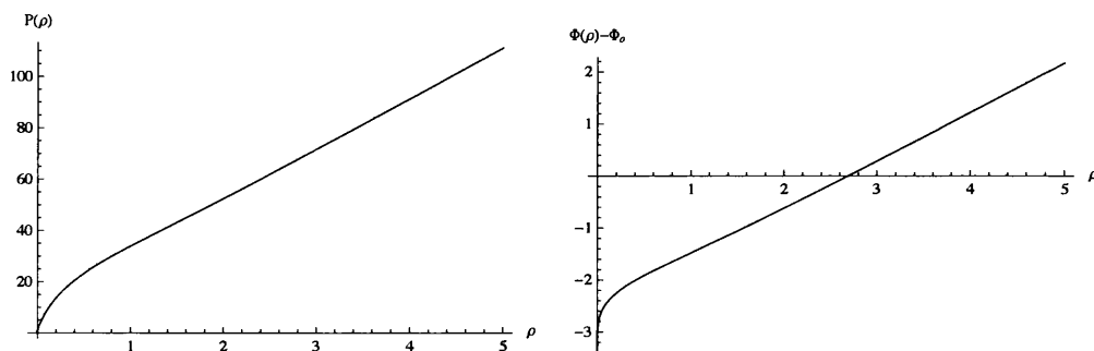
Figure 5.3: Plot of the function P(\rho) and the dilaton for the numerical solution interpolating between the IR asymptotic behaviour in (5.3.21) and the linear UV asymptotics P \sim |2\tilde{N}_c - \tilde{N}_f|\rho . The plots correspond to the values \tilde{N}_c = 20 , \tilde{N}_f = 20 , P_o = 10 and h_1 = 25.93 . Contrary to the \tilde{N}_f = 0 case, we do not have an analytic expression for the value of h_1 leading to linear dilaton asymptotics in the UV.
