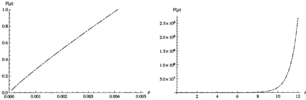
Figure 5.2: In these graphs, we plot the same numerical solution as in Figure 5.1, but we zoom in on the IR region (left) and on the UV region (right), and we compare the numerical solution (black) with the corresponding asymptotic solutions given in (5.3.21). These are plotted in red (IR solution) and in blue (UV solution).
