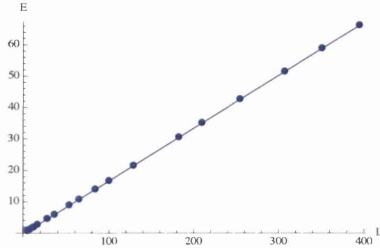
Figure 4.3: Plot of the energy E of the Wilson loop, as a function of the quark separation L . We can see a linear confining behaviour. This plot corresponds to a solution with second UV asymptotics, with \tilde{N}_c = 1 and \tilde{N}_f = 0 .
