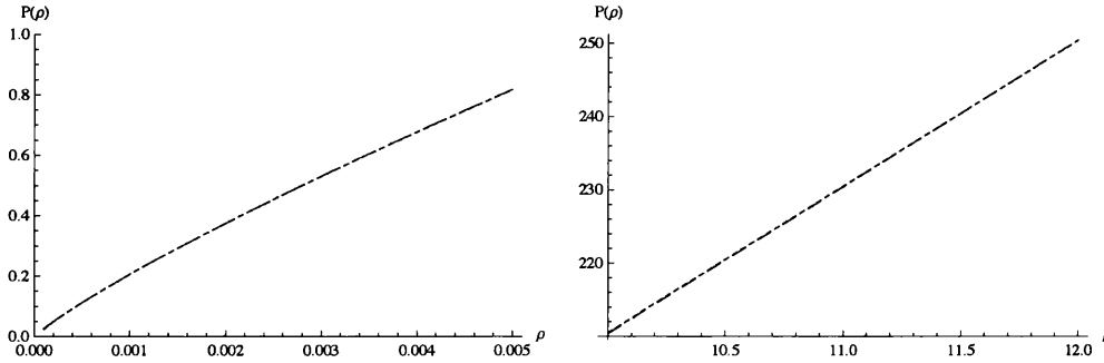
Figure 5.4: Here, we plot the same numerical solution as in Figure 5.3, but we zoom in on the IR region (left) and on the UV region (right), and we compare the numerical solution (black) with the IR asymptotic solution given in (5.3.21) and the UV asymptotic solution P \sim |2\tilde{N}_c - \tilde{N}_f|\rho . These are plotted in red (IR solution) and in blue (UV solution).
