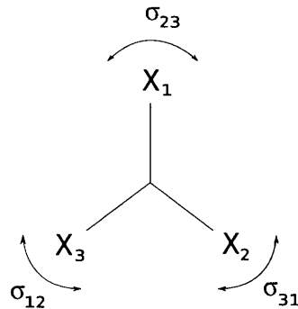
Figure 6.1: The moduli space of asymptotically conical G_2 -holonomy metrics on S^3 \times \mathbb{R}^4 has three branches permuted by the action of the group \Sigma_3 . The three G_2 -holonomy metrics are invariant under elements of order two \sigma_{ij} , which are reflections about each of the three axes. The intersection point of the three branches corresponds to the singular G_2 cone. In the notation of [126], X_1 corresponds to \lambda = 0 , X_2 corresponds to \lambda = -1 and X_3 corresponds to \lambda = 1 .
