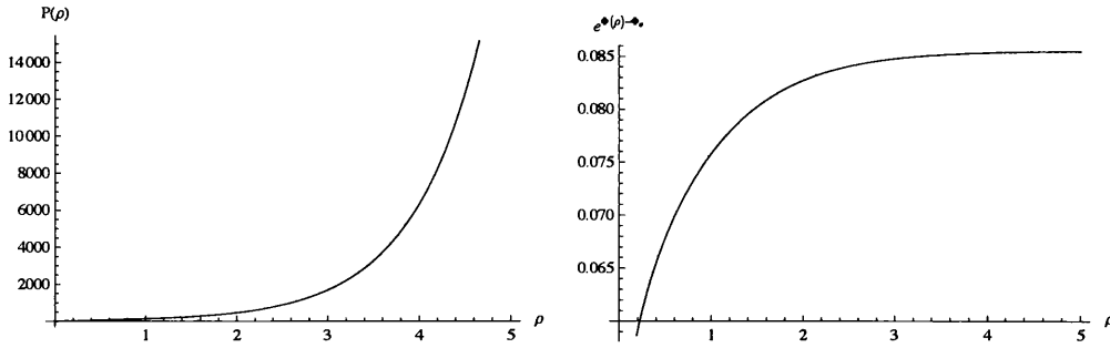
Figure 5.1: Plot of the function P(\rho) and the dilaton for the numerical solution interpolating between the two asymptotic behaviours in (5.3.21). The plots correspond to the values \tilde{N}_c = 10 , \tilde{N}_f = 20 , c = 30 , and h_1 = 100 .
