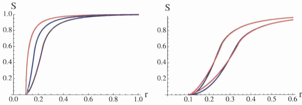
Figure 7.1: We show plots of the function S for the flat measure on the left. The red curve is the singular profile, the blue one is for \delta = 0.15 and the purple one is for \delta = 0.4 . On the right, we plot, for \delta = 0.5 and \delta = 1 , S for the flat measure (red) and the peaked one (blue) and we see that there is almost no difference.
