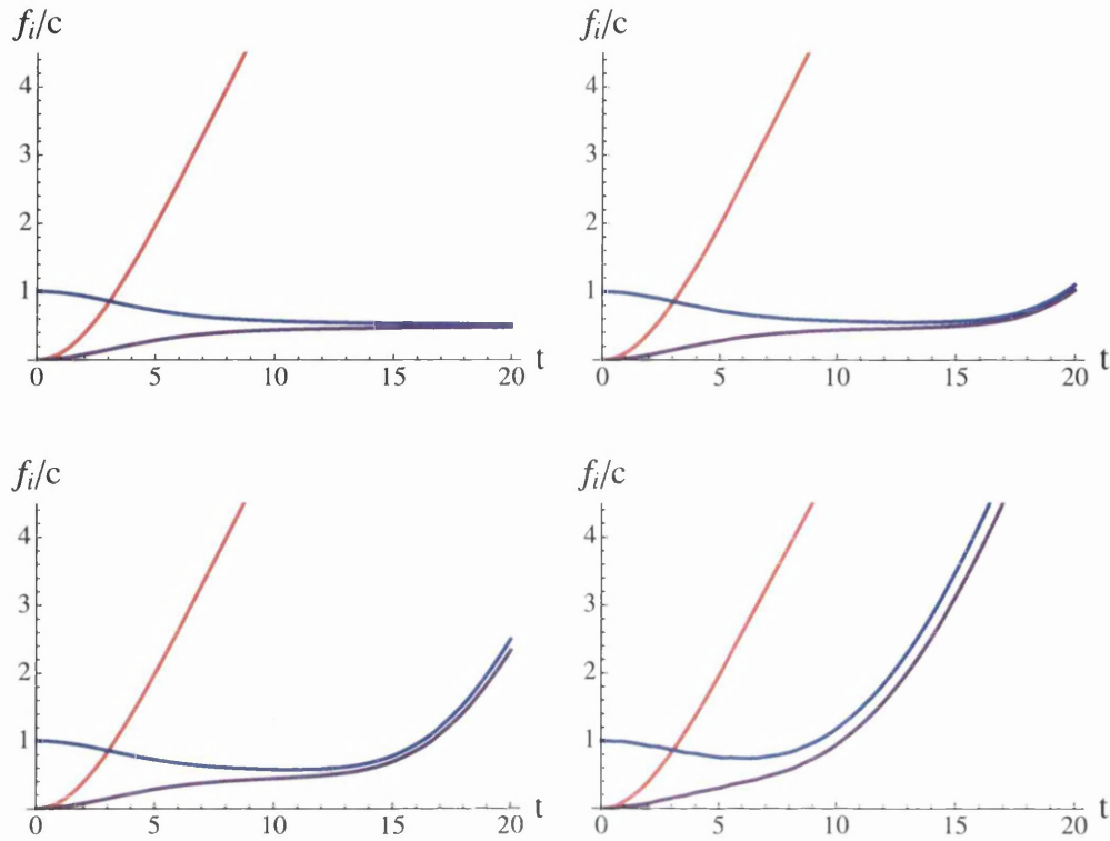
Figure 6.3: Plots of the functions c^{-1}f_i for the X_{31} solution for different values of c . f_1 is in red, f_2 in purple and f_3 in blue. The factor c^{-1} is there for normalisation purposes. From the top left to the bottom right, the values of c are increasing and are 0.125 (the exact minimum value), 0.125001, 0.12501 and 0.126. The first plot is the Maldacena-Nastase solution.
