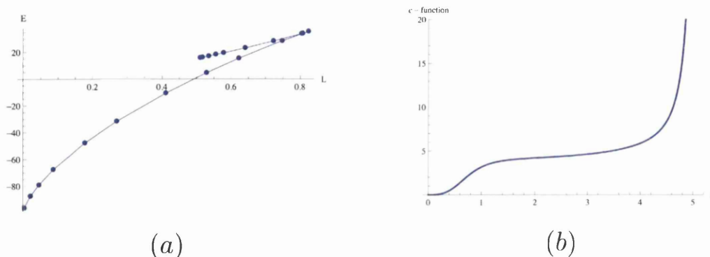
Figure 4.4: In (a) we plot E vs. L for a solution with third UV asymptotics. In (b) we plot the corresponding c -function for this solution. Notice the plateau it shows. Both figures are with \tilde{N}_c = 1 and \tilde{N}_f = 0 .
