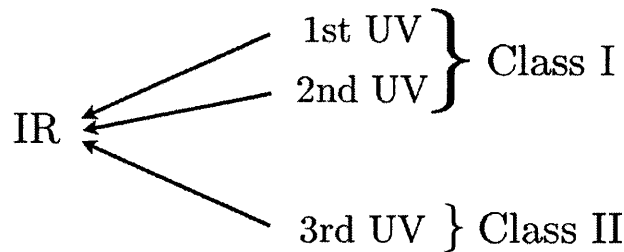
Figure 4.2: On this picture is represented schematically the classification of solutions in the \mathbb{H}_2 \times \widetilde{SL}_2 case and their RG flow.
