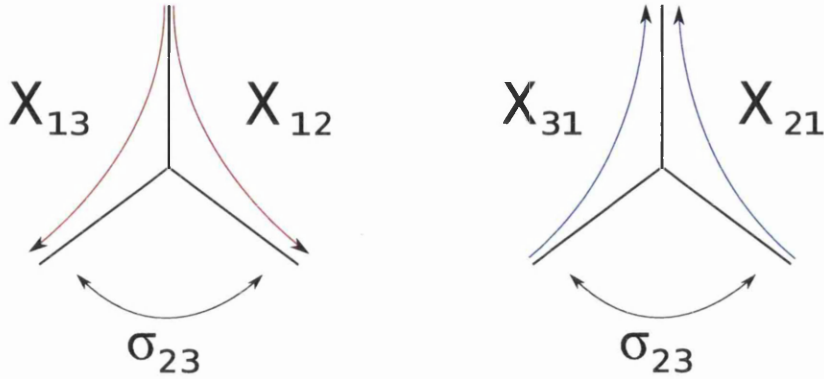
Figure 6.5: On the left: the solutions X_{13} and X_{12} interpolate continuously between the G_2 manifold X_1 with flux and the G_2 manifolds X_3 and X_2 with branes, respectively. The two solutions are related by the \mathbb{Z}_2 symmetry \sigma_{23} and both have topology of X_1 \cong S^3 \times \mathbb{R}^4 . On the right: the solution X_{31} interpolates continuously between the G_2 manifold X_3 with flux and the G_2 manifold X_1 with branes, while the solution X_{21} interpolates between the G_2 manifold X_2 with flux and the G_2 manifold X_1 with branes. The two solutions are related by the same \mathbb{Z}_2 symmetry \sigma_{23} , however X_{31} has the topology of X_3 \cong S^3 \times \mathbb{R}^4 while X_{21} has the topology of X_2 \cong S^3 \times \mathbb{R}^4 .
