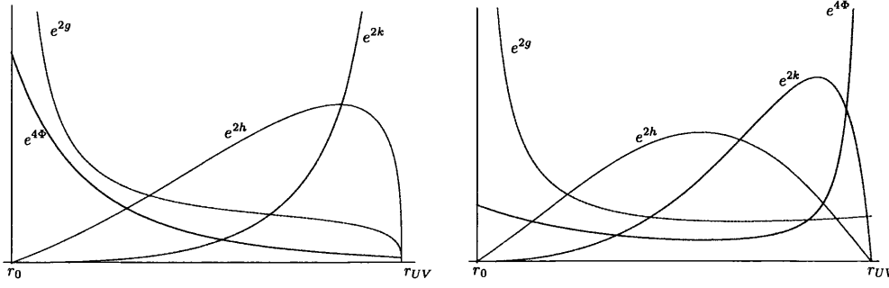
Figure 4.1: Plots of the functions e^{2g} , e^{2h} , e^{2k} and e^{4\Phi} . On the left, the plots are of class I solutions, while on the right they are of class II.
