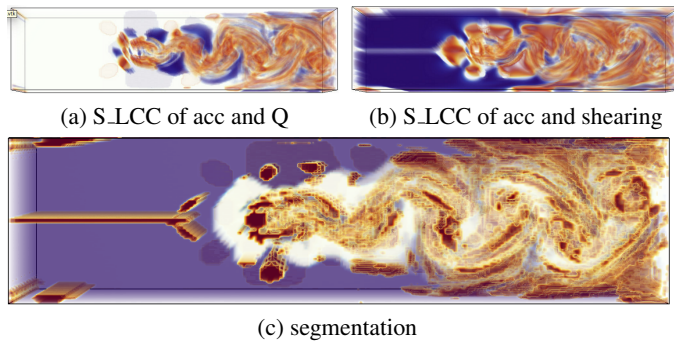
Fig. 5: Spatial LCC of acceleration and Q (a) vs acceleration and shearing (b) and the segmentation result for three pairs of these attributes (c). In (c), red regions correspond to places where the correlation between acceleration and Q is the strongest. White regions visualize the places where acceleration and shearing has the highest value of correlation, and purple segments correspond to the regions where correlation between shearing and Q is the strongest.
