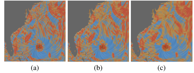
Fig. 14: The effect of spatial kernel size, r , on Lagrangian ST_LCC. From the left image to right, the r values for the results are 3, 5, and 10, respectively.
