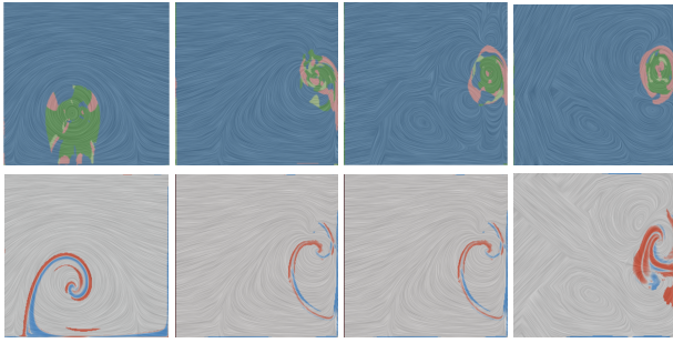
Fig. 9: The top row shows the ranking based segmentation for the spatial correlation between pressure and other attributes over time (from left to right). The green color indicates the regions where the correlation of pressure and vorticity is the highest, the pink color corresponds to the pair of pressure and kinetic energy, and blue for the pair of pressure and shearing. The second row shows the result of ST_LCC for acceleration and kinetic energy. The results highlight regions similar to the FTLE ridges. The spatial kernel size is r = 3 and the temporal kernel size is h = 40 .
