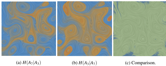
Fig. 8: The comparison of conditional entropy for norm of the Jacobian ( A_7 ) vs. \lambda_2 ( A_3 ). Blue-white-red color coding is applied to (a) and (b), while for (c), light green indicates H(A_7|A_3) < H(A_3|A_7) while blue means H(A_3|A_7) < H(A_7|A_3) .
