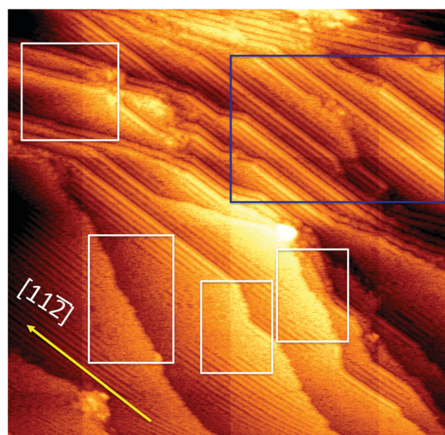
Fig. 5 STM image, 75 nm \times 75 nm, showing regular staple rows in regions with parallel [11\bar{2}] steps. Steps not along the major crystallographic directions appear to be less stable and thiolates near such irregular steps are in a disordered state.
