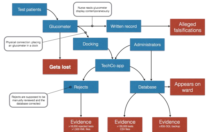
Figure 3. Diagram presented in court (anonymized) to show key sources of evidence. It was originally sized as A4 — for the present paper the details are less important than noting the complexity, in particular with no end-to-end checking of integrity. The police made digitally signed copies of Evidence 1, 2 and 3, but signing occurred after the police had manually copied the data, so it could only be used to show the data had not changed after it had been collected. The digital signatures did not assure that the data was what it was claimed to be. This diagram does not show Abbott’s modifications of data, which only became apparent after the diagram was submitted to the court.
