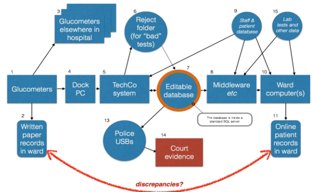
Figure 2. Diagram presented in court (anonymized) originally sized as A4; the smaller reproduction here serves to indicate the complexity of the network, but note that Box 8 in the figure contains unknown further software. The basic problem was that there were discrepancies between the paper records (bottom left) and the final computer records (bottom right). Note that not all relevant systems are Abbott's (the 'middleware' box may, and probably does, contain further complications). Numbers in the figure were used to cross reference this diagram to other expert evidence.
